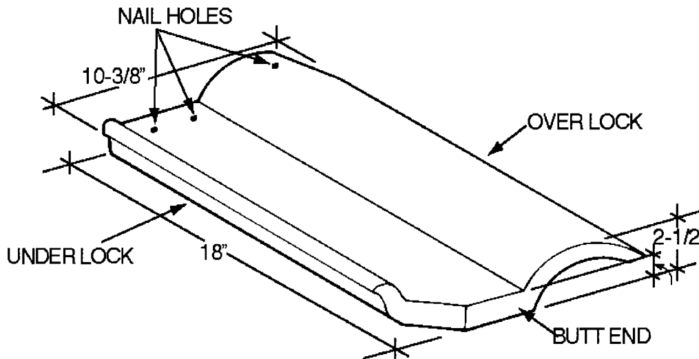
MONIER LIFETILE SPANISH 'S' CONCRETE ROOF TILE
