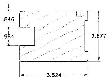
38 POCKET JAMB STILE
