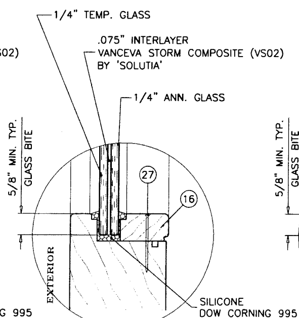
GLAZING TYPE 'B'
