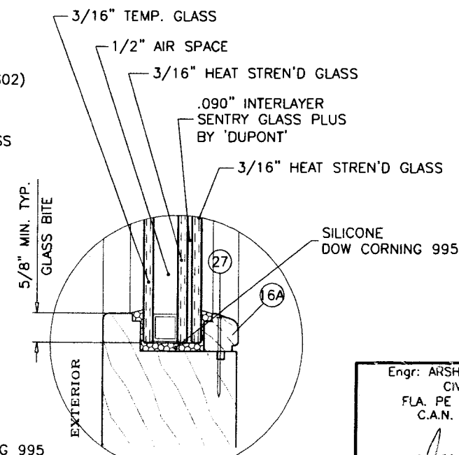
GLAZING TYPE 'D'
