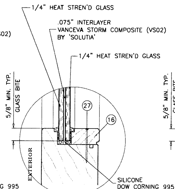
GLAZING TYPE 'C'
