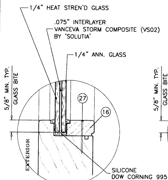
GLAZING TYPE 'A'
