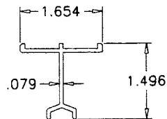
20 EXTRUDED GUIDING RAIL
