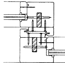
MTG. STILES WITH REINFORCING
