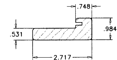
40 POCKET STILE HOOK
