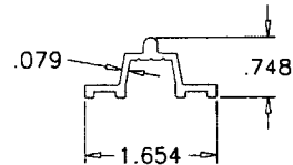
21 EXTRUDED RUNNING RAIL
