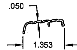
③ #8004C 6063-T5 OS SILL COVER
