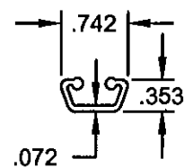
(28) #8020A 6063-T6 GEAR HINGE, COVER
