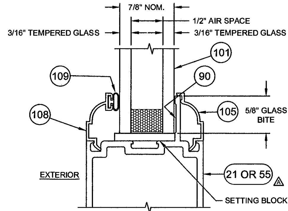
GLAZING DETAIL I.G. GLASS
