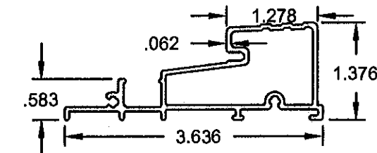
⑩ #8056 6063-T6 OUT-SWING LOW SILL
