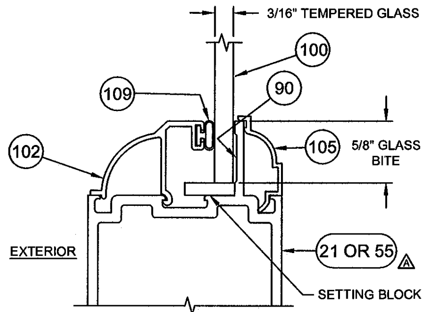
GLAZING DETAIL MONOLITHIC GLASS
