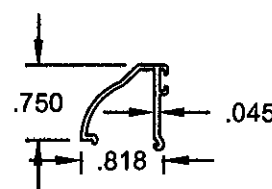
(107) #8023A 6063-T5 7/16" BEAD
