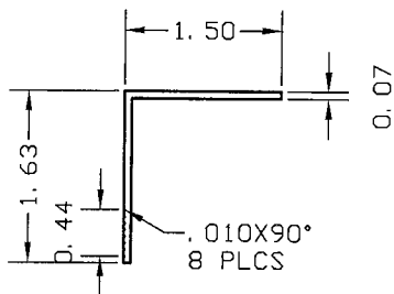
3- HW RETAINER 6063-T5 ALUMINUM ALLOY
