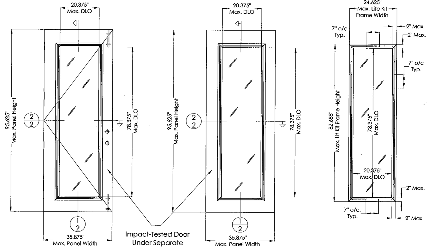
SINGLE-GLAZED SWINGING DOOR PANEL
