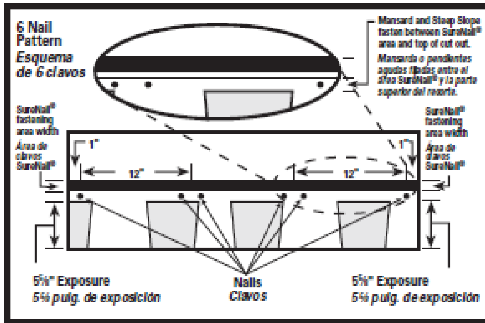
SLOPE GREATER THAN 21:12
