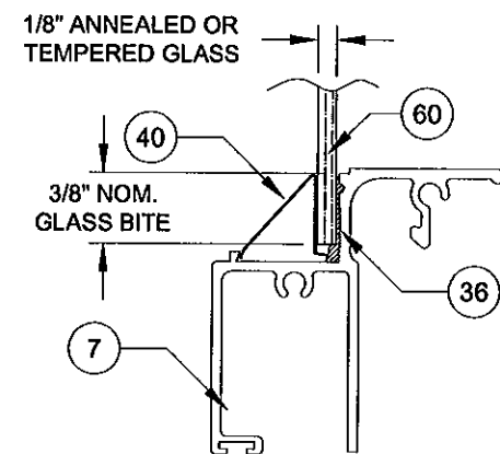
1/8" GLAZING DETAIL GLASS TYPES A & B
