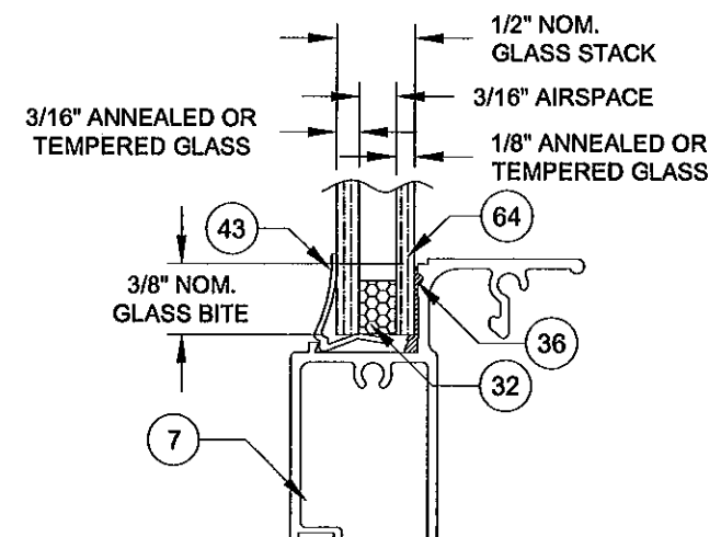
1/2" I.G. GLAZING DETAIL GLASS TYPES H & J
