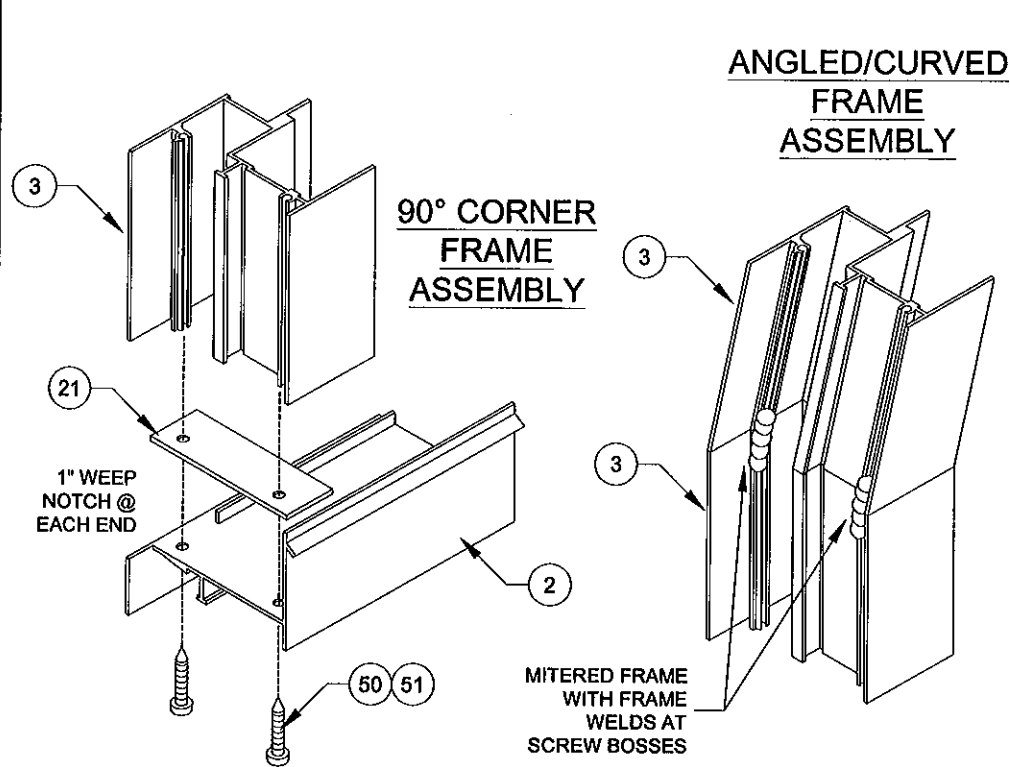
ASSEMBLY DETAILS FOR FLANGE FRAME CORNERS
