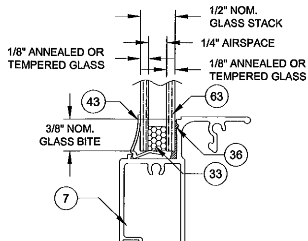
1/2" I.G. GLAZING DETAIL GLASS TYPES G & I
