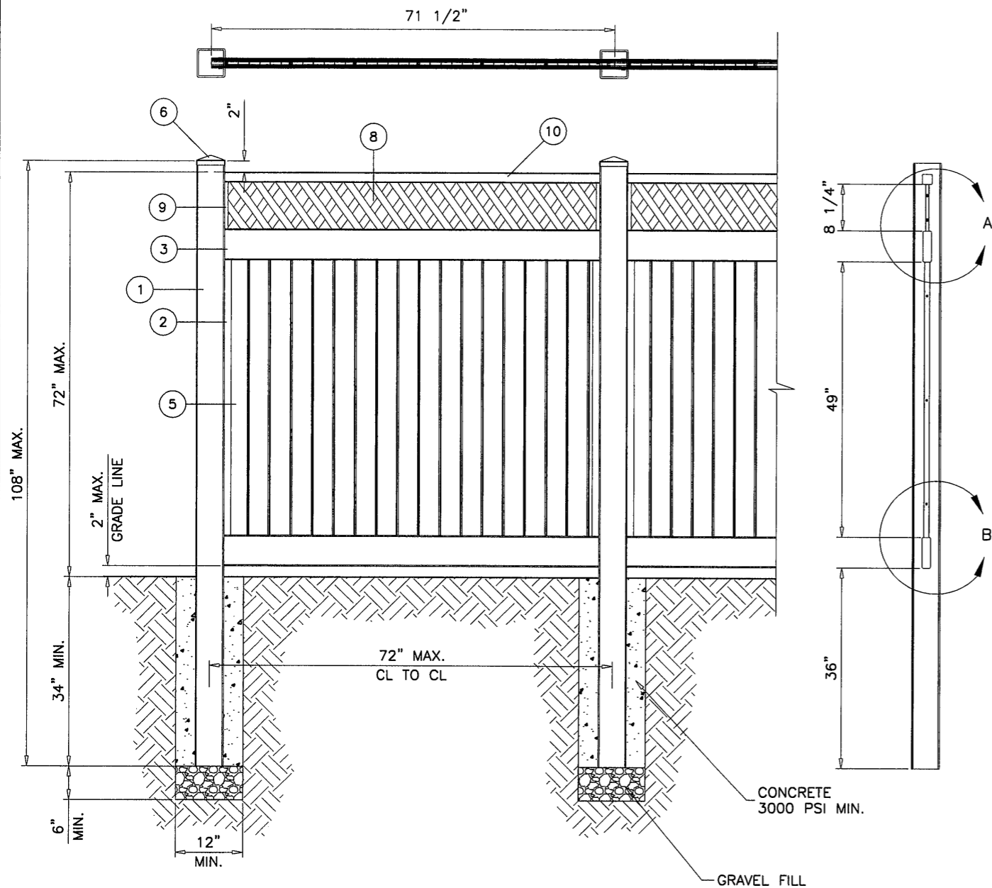
TYPICAL ELEVATION 1/2" = 1'-0"
