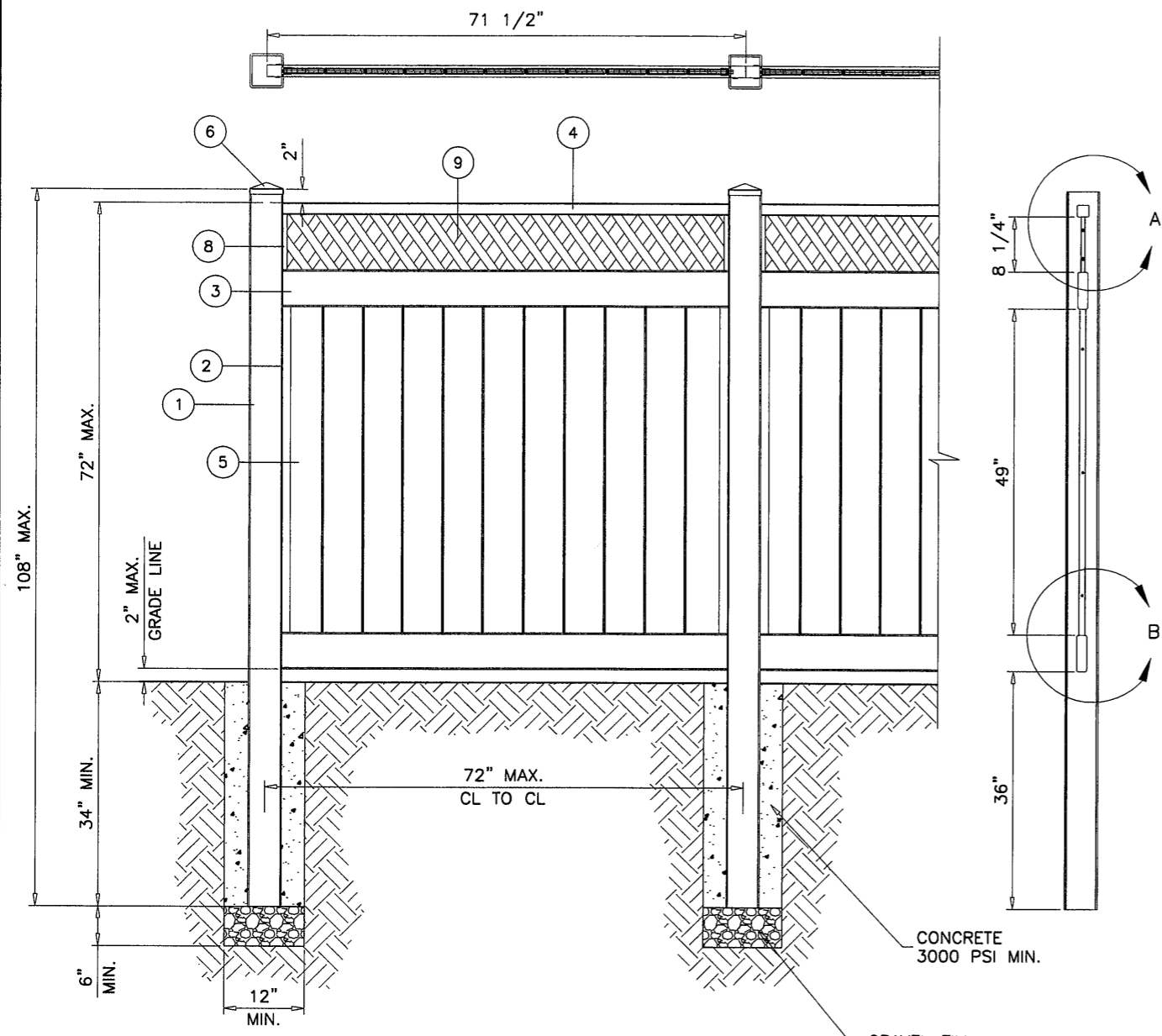
TYPICAL ELEVATION 1/2" = 1'-0"
