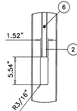
DETAIL 'B' 1" = 1'-0"
