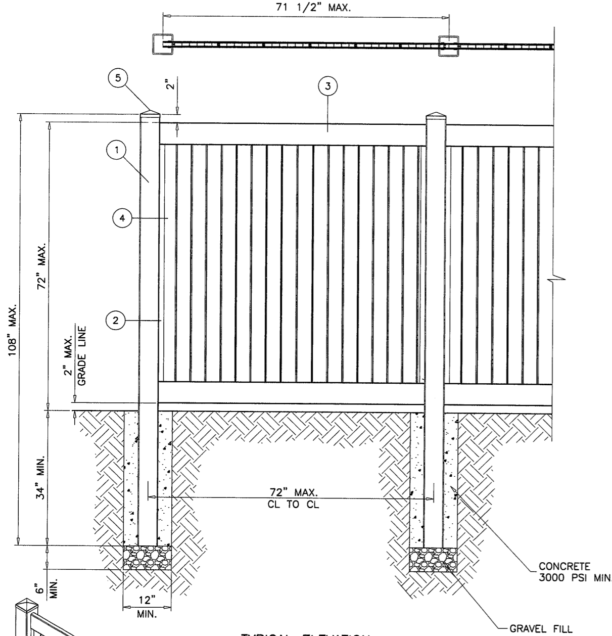
TYPICAL ELEVATION 1/2" = 1'-0"
