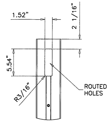
DETAIL 'A' 1" = 1'-0"
