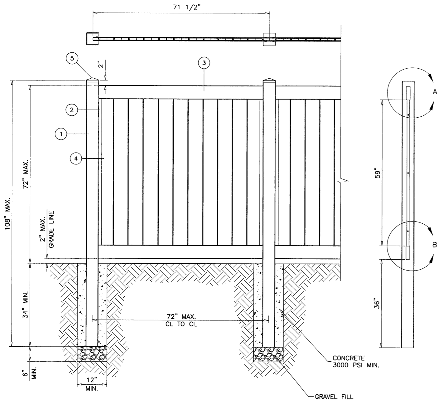
TYPICAL ELEVATION 1/2" = 1'-0"
