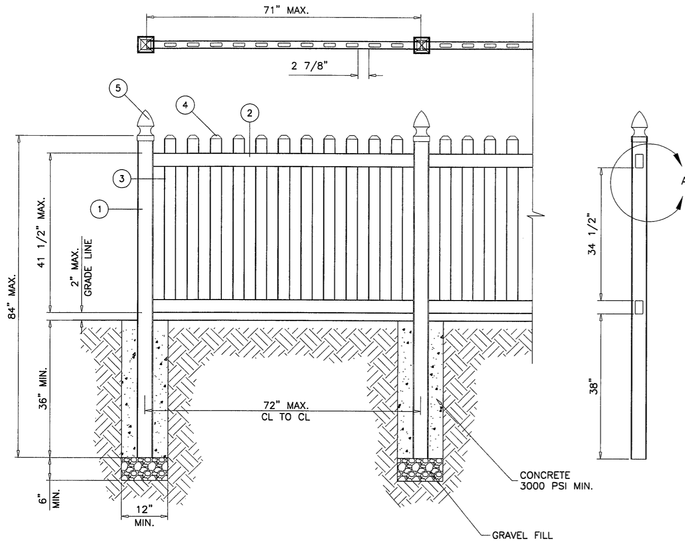
TYPICAL ELEVATION 1/2" = 1'-0"
