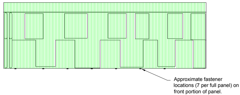
Figure 2. Fastener Locations DECRA Tile, Shake and Shingle Plus A-1, A-2 and A-4 Perimeter Conditions
