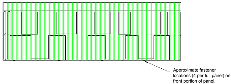
Figure 1. Fastener Locations DECRA Tile, Shake and Shingle Plus A-1, A-2 and A-4 Field Conditions
