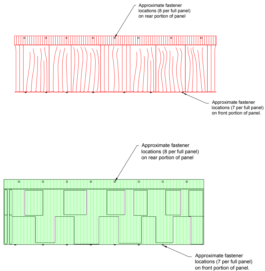
Figure 3. Fastener Locations DECRA Shake Plus and Shingle Plus A-3 Deck
