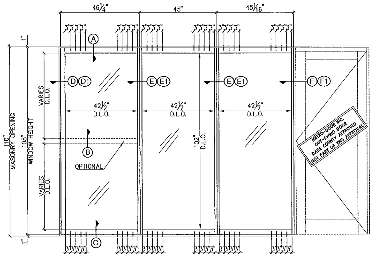
FIXED WINDOW ELEVATION EXTERIOR VIEW
