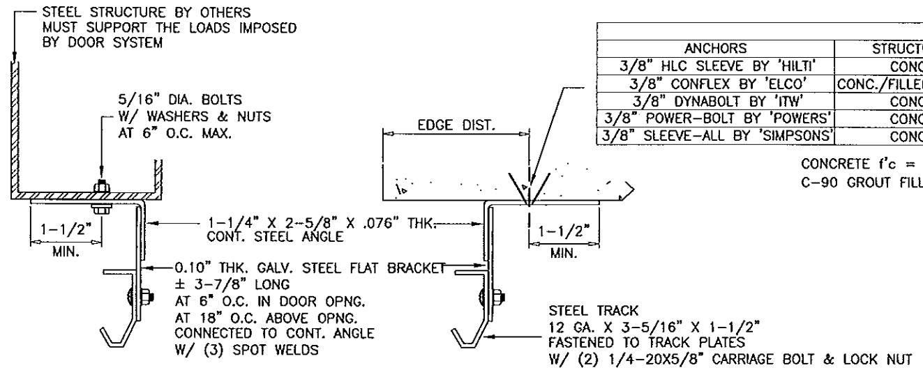
TRACK INSTALLATION
