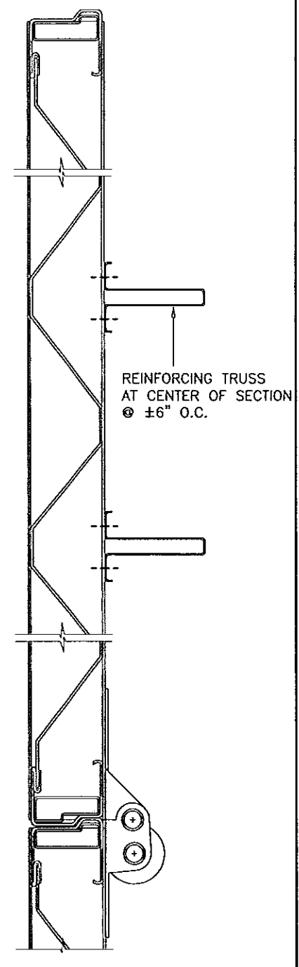
ALL TOP SECTIONS REINFORCING
