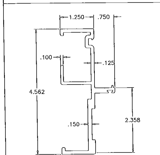
CGI-507 DOOR FRAME HEAD/SILL
