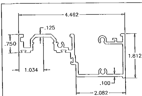
CGI-507 DOOR FRAME HEAD/SILL
