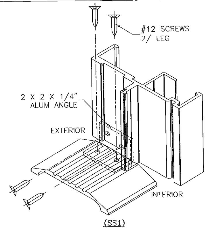
ADA SILL CORNER DETAIL
