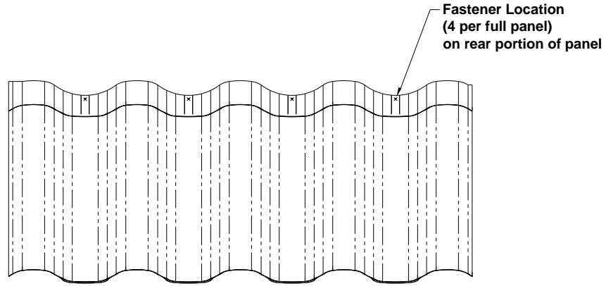
FIGURE 3 FASTENER LOCATIONS DECRA VILLA TILE A(2) DECK
