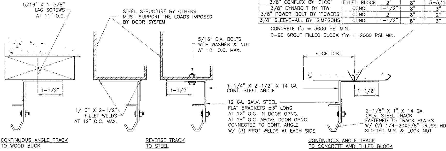
ALTERNATE TRACK INSTALLATION
