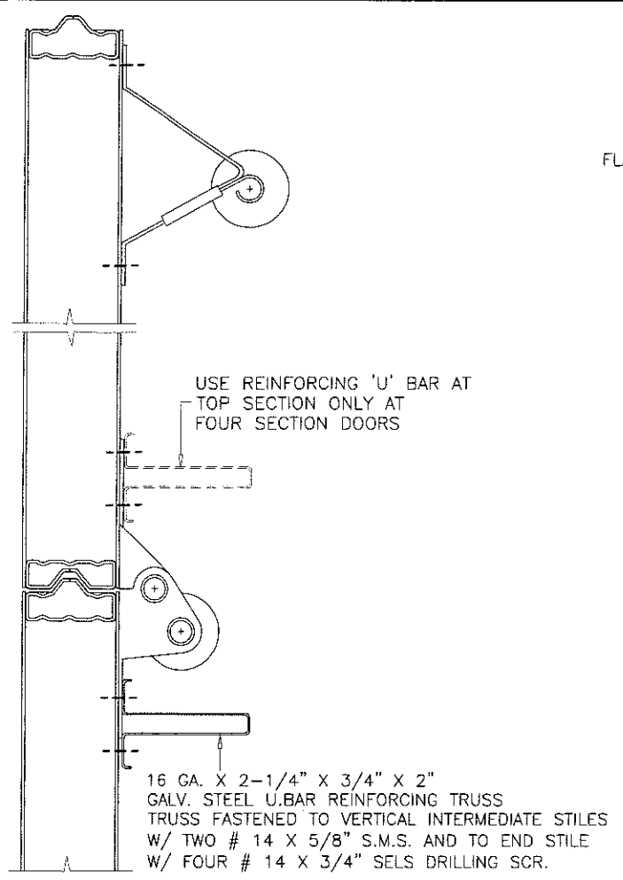
TOP SECTION
