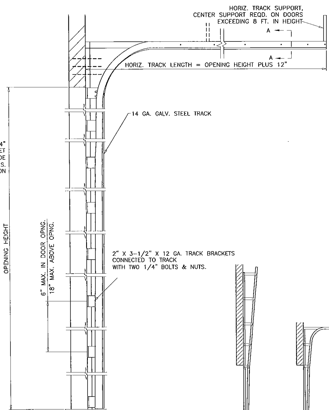
TRACK CONFIGURATION
