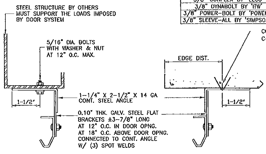
TRACK INSTALLATION
