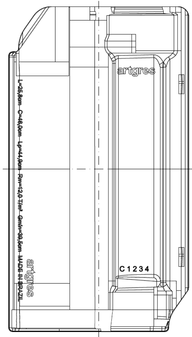
AMERICAN SPANISH 'S' CLAY ROOF TILE
