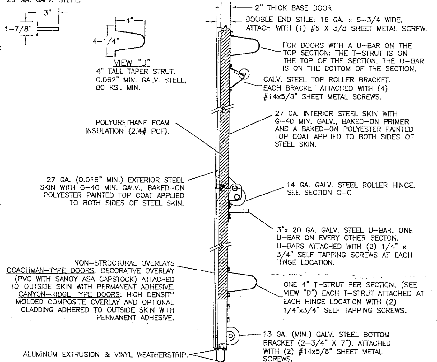
SECTION A-A (SIDE VIEW)
