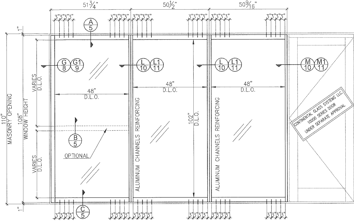
FIXED WINDOW ELEVATION EXTERIOR VIEW
