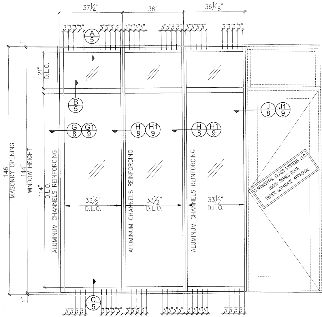
FIXED WINDOW ELEVATION EXTERIOR VIEW
