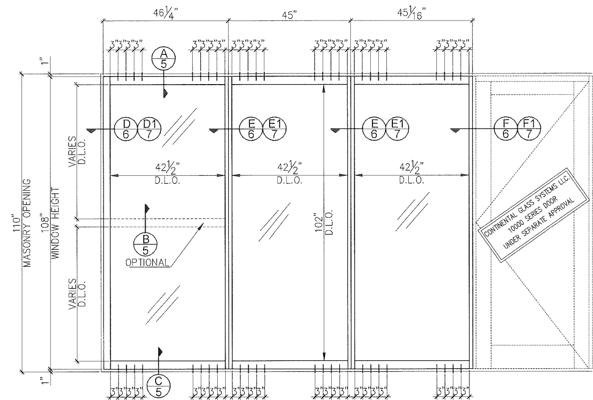
FIXED WINDOW ELEVATION EXTERIOR VIEW
