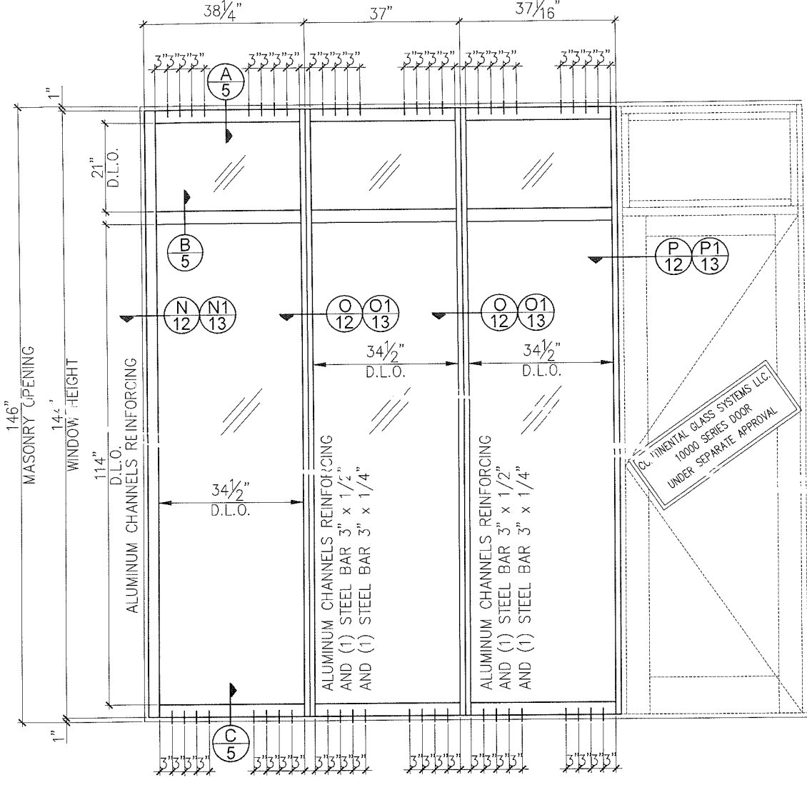
FIXED WINDOW ELEVATION EXTERIOR VIEW
