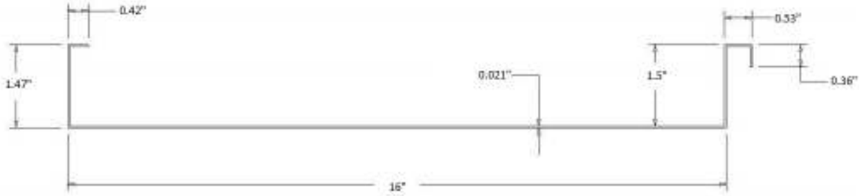
UNA-CLAD UC-3 Copper Panel
