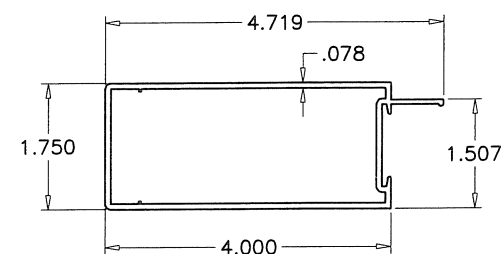
9 LEAF HINGE STILE
