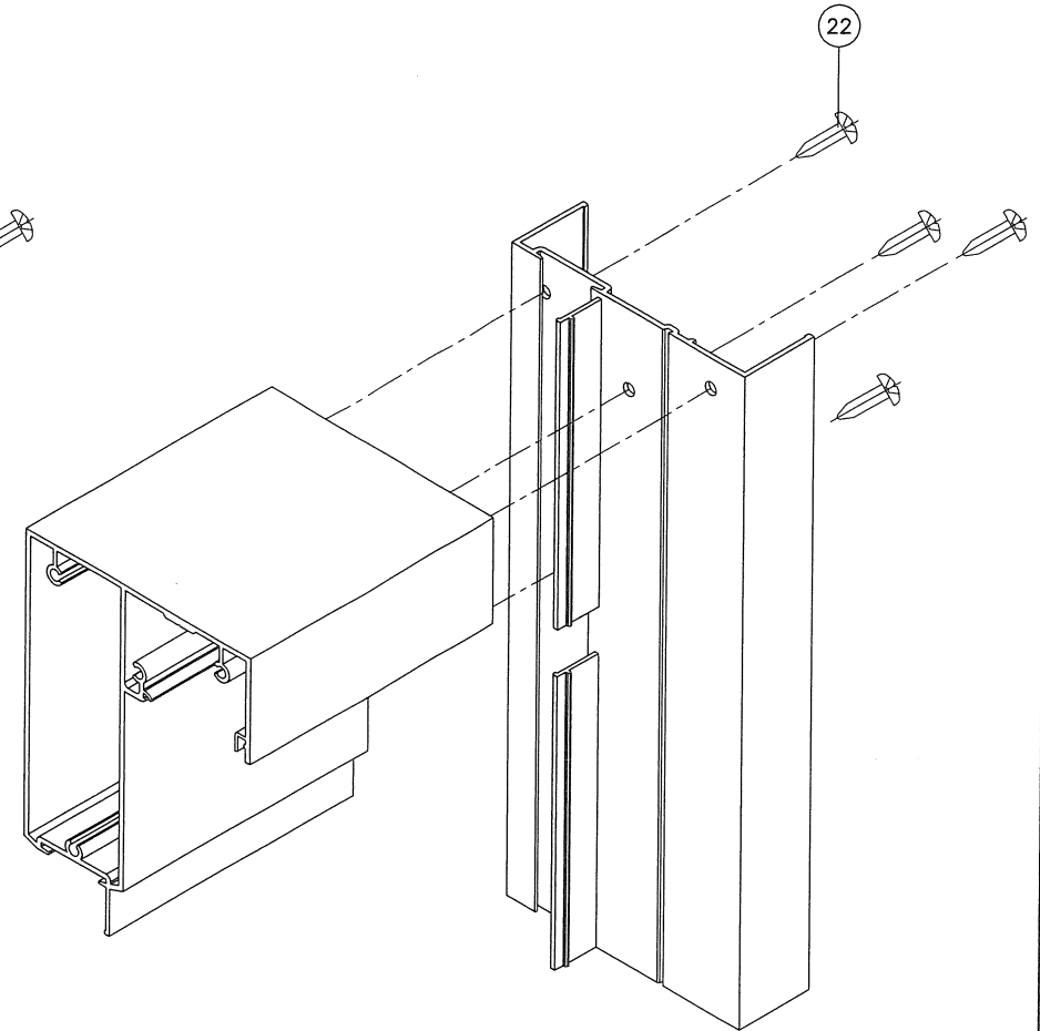
SIDELITE MULLION SLIP ON JAMB CORNER
