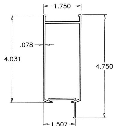
⑦ LEAF TOP/BOTTOM RAIL
