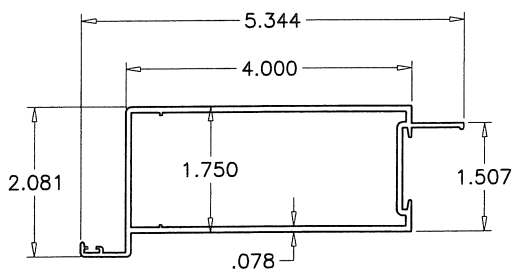
10 LEAF LOCK STILE
