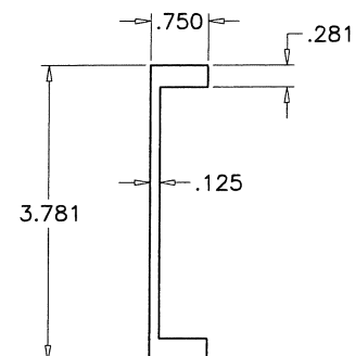
18 SIDELITE MULLION REINFORCING
