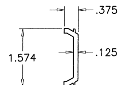
13 LEAF CLAMP HINGE BACK-UP PLATE
