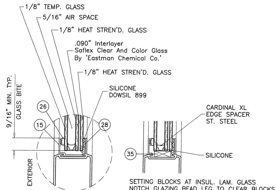
GLASS TYPE 'G3'
