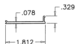
② FRAME COVER
