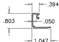
14A GLAZING BEAD 7/16" GLASS
