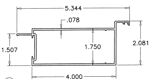
11 LEAF ASTRAGAL STILE
