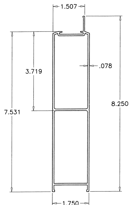
9" BOTTOM RAIL
