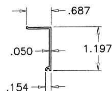
(16) SNAP COVER
