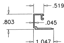
14 GLAZING BEAD 5/16" GLASS
