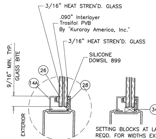
GLASS TYPE 'G2'
