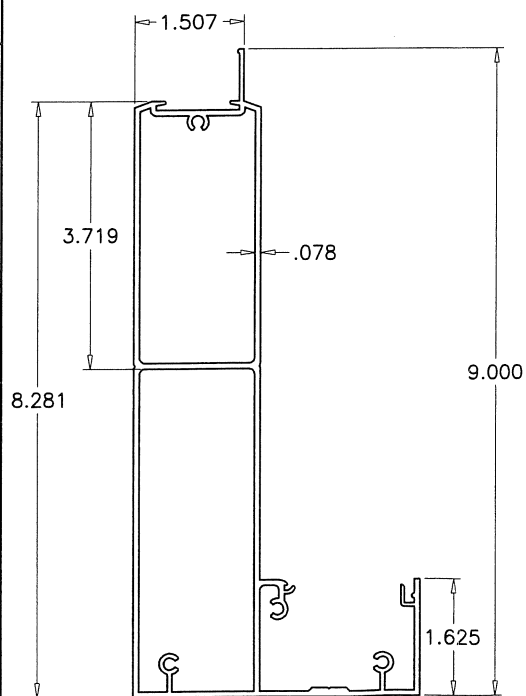
4A SIDELITE 9" BOTTOM FRAME
