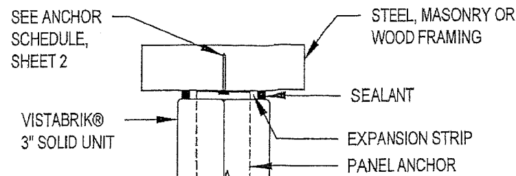
PANEL ANCHOR RESTRAINT DETAIL SCALE: 3" = 1'-0"
