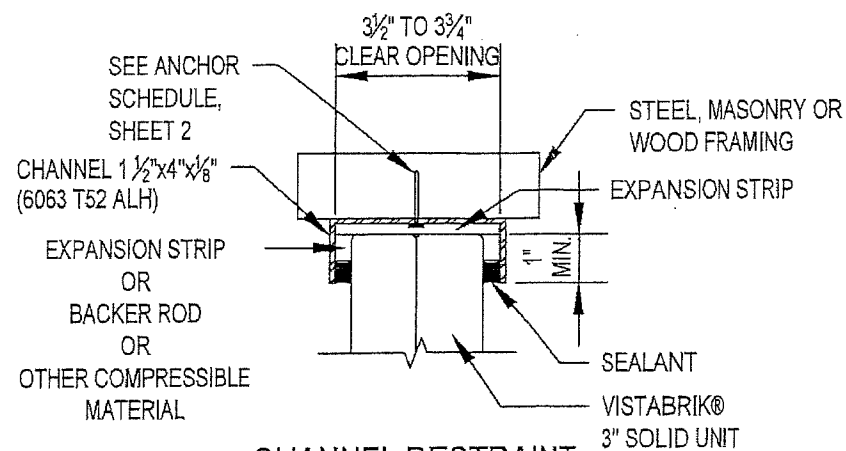
CHANNEL RESTRAINT DETAIL SCALE: 3" = 1'-0"
