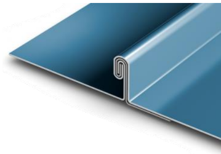
180° DOUBLELOCK
