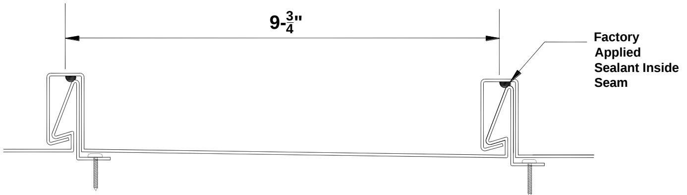
UC-4 METAL ROOF PANEL
