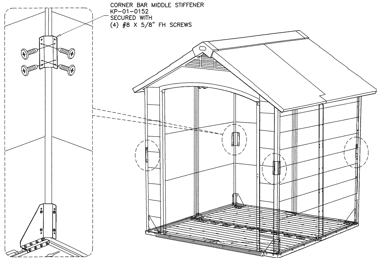
CORNER BAR MIDDLE STIFFENER
