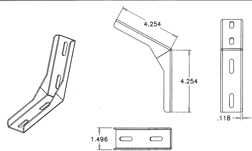
SIDE + ROOF JOINT (KP-01-0104) (GALV. STEEL) (2 REQD.)
