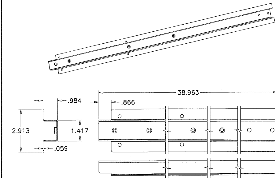
ROOF BEAM (KP-01-0105) (GALV. STEEL) (3 REQD.)
