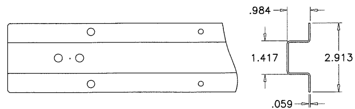
REAR WALL BEAM (KP-01-0131) (GALV. STEEL) (1 REQD.)
