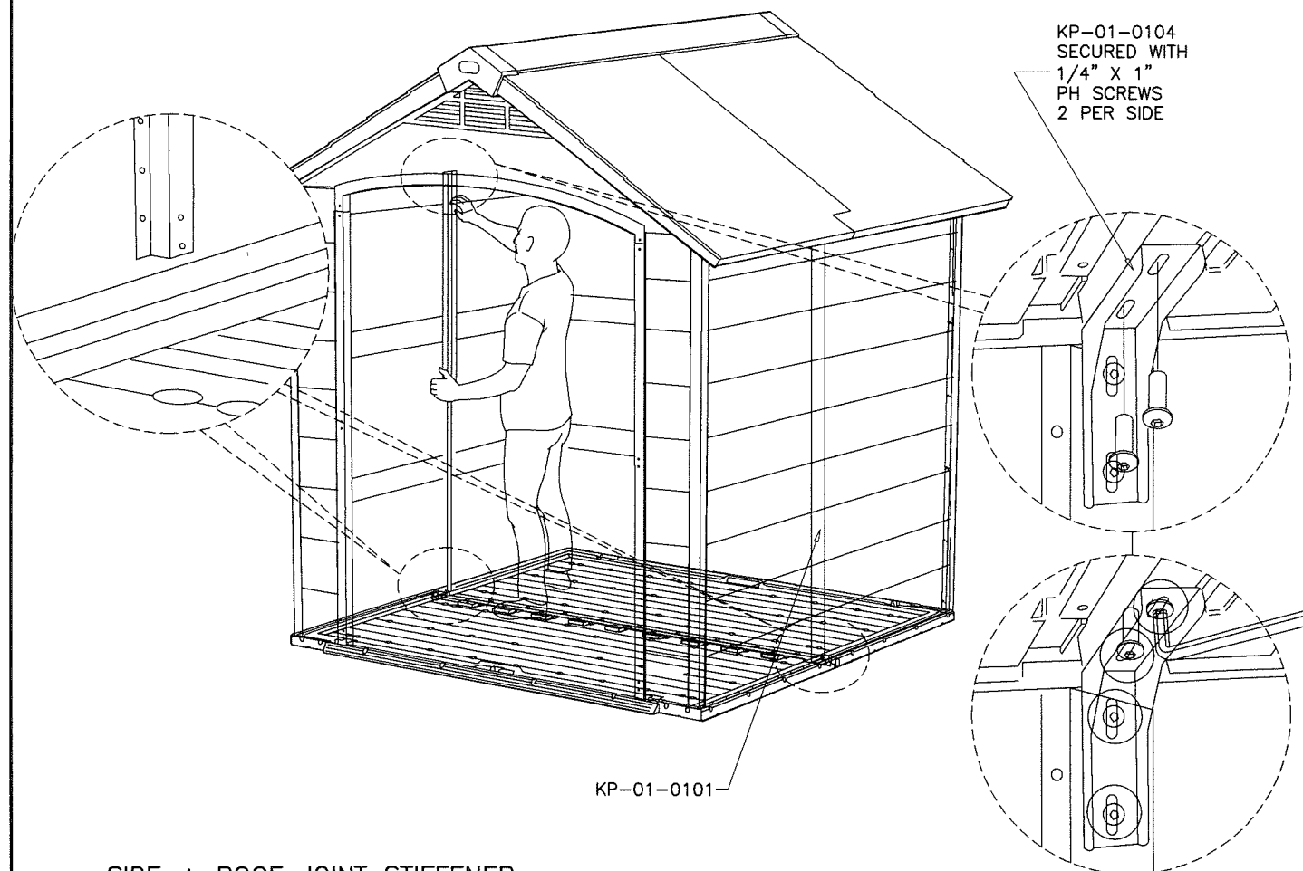
SIDE + ROOF JOINT STIFFENER
