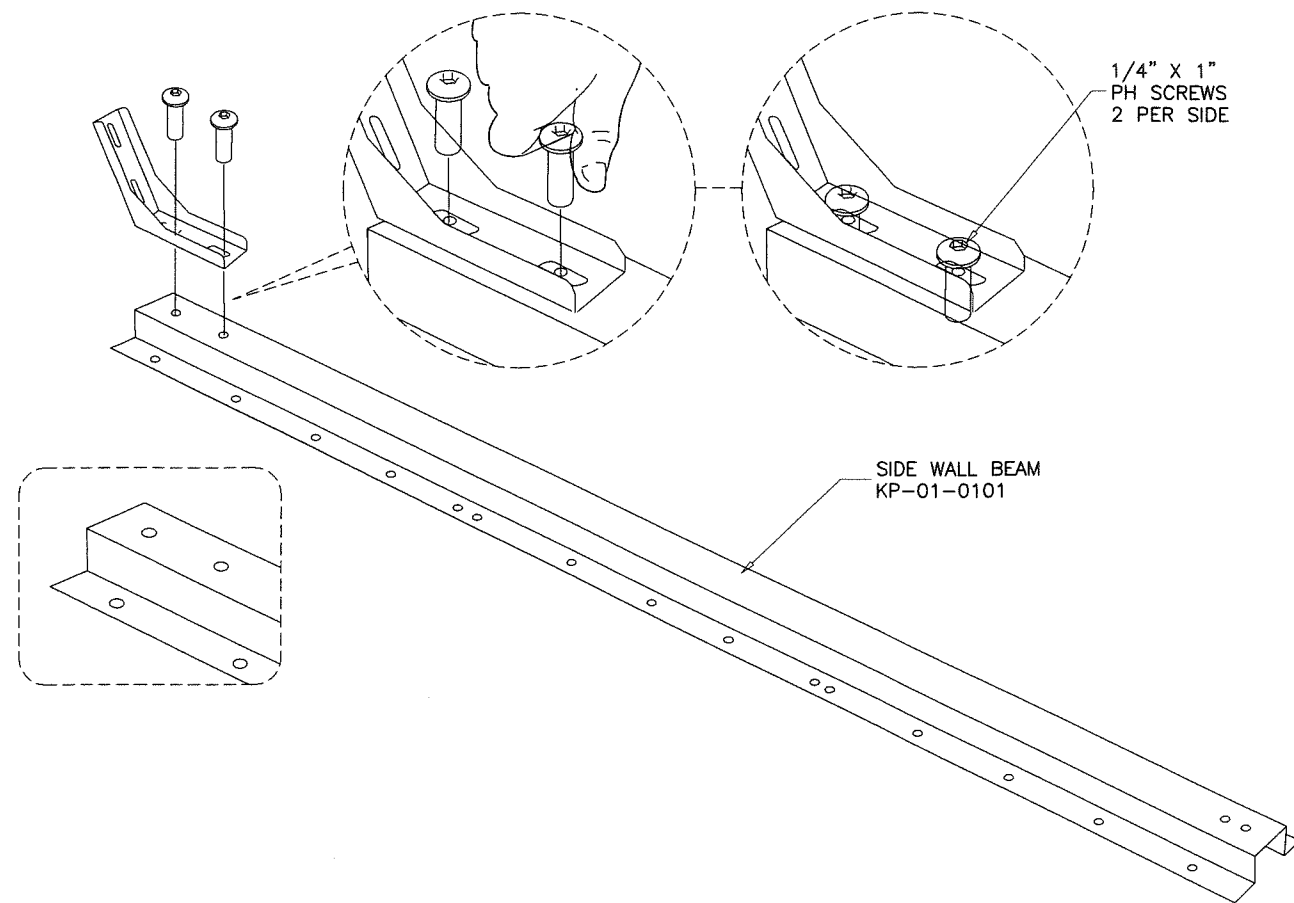
SIDE WALL BEAM
