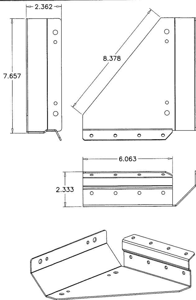
BOTTOM CORNER STIFFENER (KP-01-0112) (GALV. STEEL) (2 REQD.)
