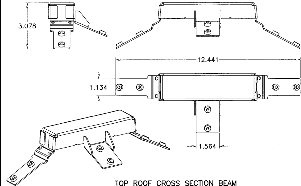
TOP ROOF CROSS SECTION BEAM (KP-01-0108) (GALV. STEEL) (1 REQD.)
