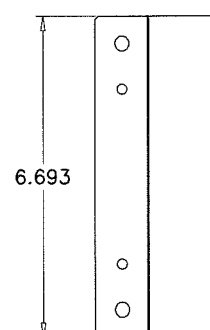
TOP CORNER STIFFENER (KP-01-0111) (GALV. STEEL) (2 REQD.)
