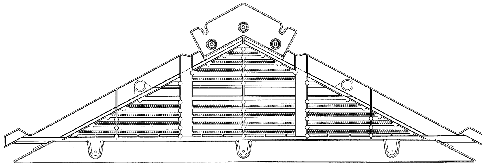
VENT (POLYPROPYLENE) (2 REQD.)
