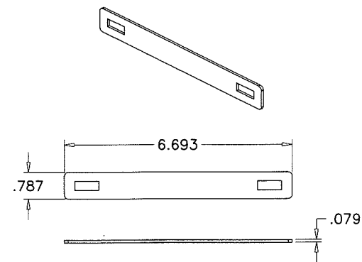
CORNER STIFFENER COLLECTIVE WASHER (KP-01-0145) (GALV. STEEL) (-)
