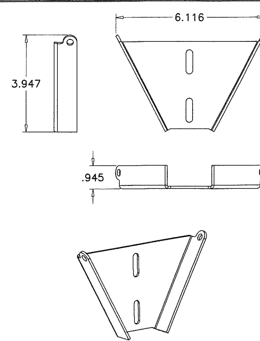
SIDE + ROOF JOINT (KP-01-0132) (GALV. STEEL) (1 REQD.)
