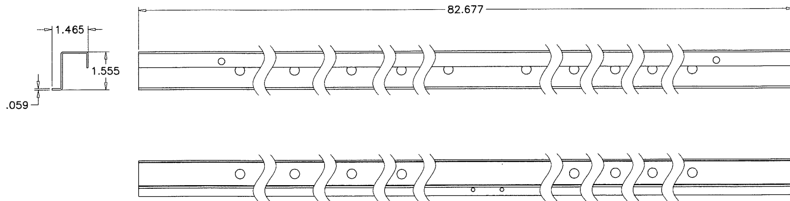
TILE SUPPORT (GALV. STEEL) (2 REQD.)
