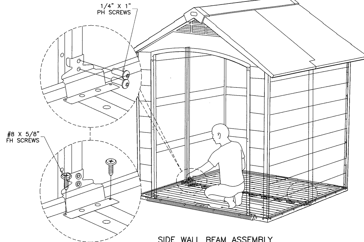
SIDE WALL BEAM ASSEMBLY
