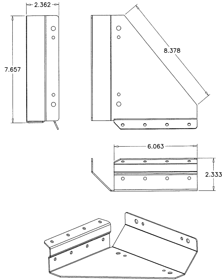
BOTTOM CORNER STIFFENER (KP-01-0113) (GALV. STEEL) (2 REQD.)
