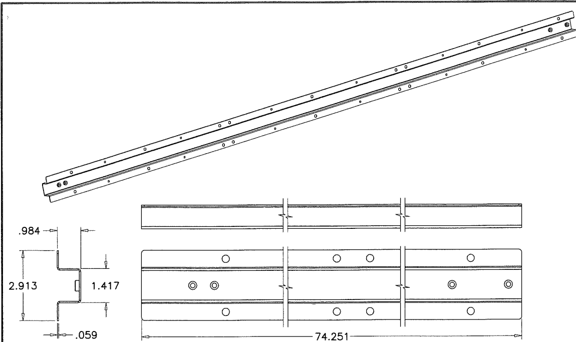
SIDE WALL BEAM (KP-01-0101) (GALV. STEEL) (3 REQD.)
