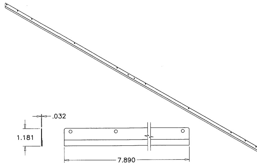
DOOR OVERLAP PLATE (KP-01-0117) (GALV. STEEL) (-)
