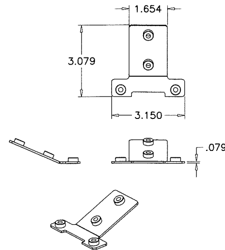
PORTAL SLOPE BEAM BOTTOM BRACKET (KP-01-0143) (GALV. STEEL) (1 REQD.)
