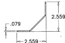
CORNER BAR MIDDLE STIFFENER (KP-01-0152) (GALV. STEEL) (4 REQD.)
