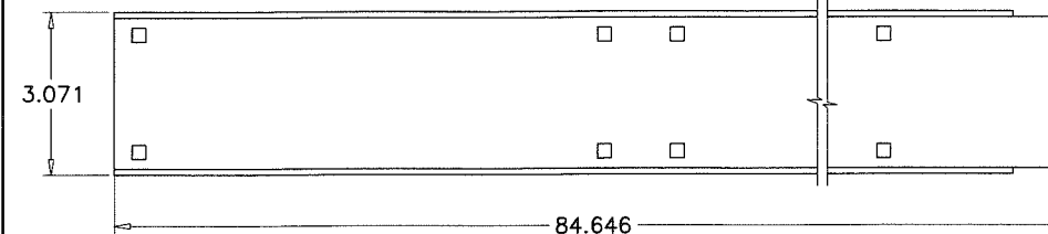
REAR WALL OPPOSITE PLATE (KP-01-0148) (GALV. STEEL) (-)
