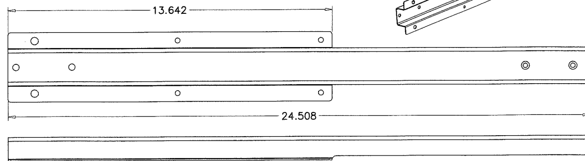
SIDE WALL BEAM EXTENSION (PEM S 0420-1) (GALV. STEEL) (1 REQD.)
