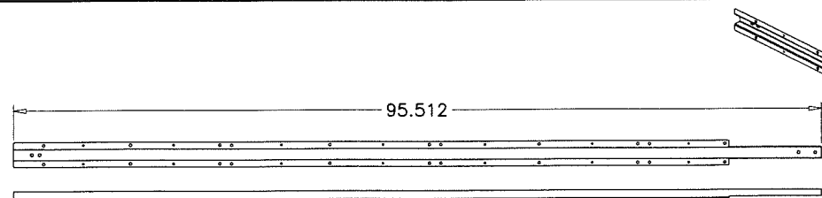
SIDE WALL BEAM EXTENSION (PEM S 0420-1) (GALV. STEEL) (1 REQD.)
