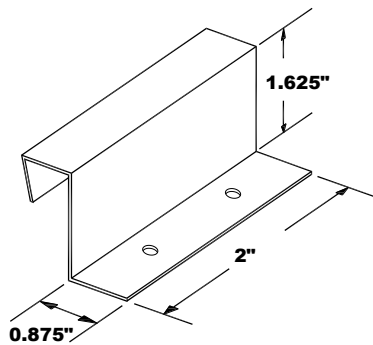
150 FIXED CLIP
