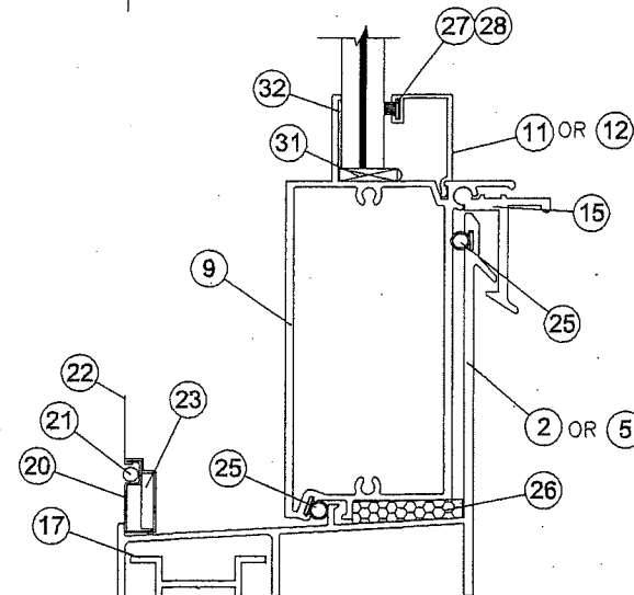
A 6 VERTICAL CROSS SECTION TWIN UNIT
