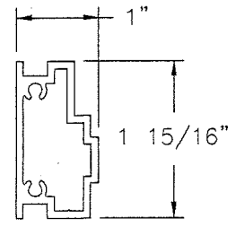
35 SHEAR BLOCK ALUMINUM 6063-T6 .090" THICK
