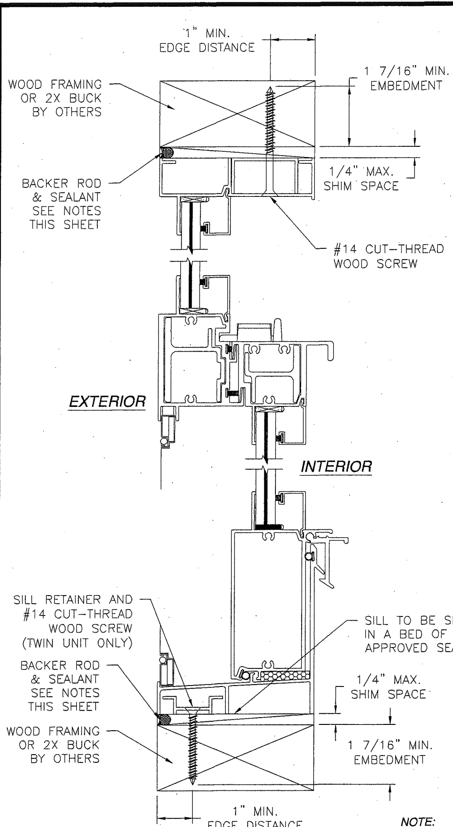
A/7 VERTICAL CROSS SECTION WOOD FRAMING OR 2X BUCK INSTALLATION
