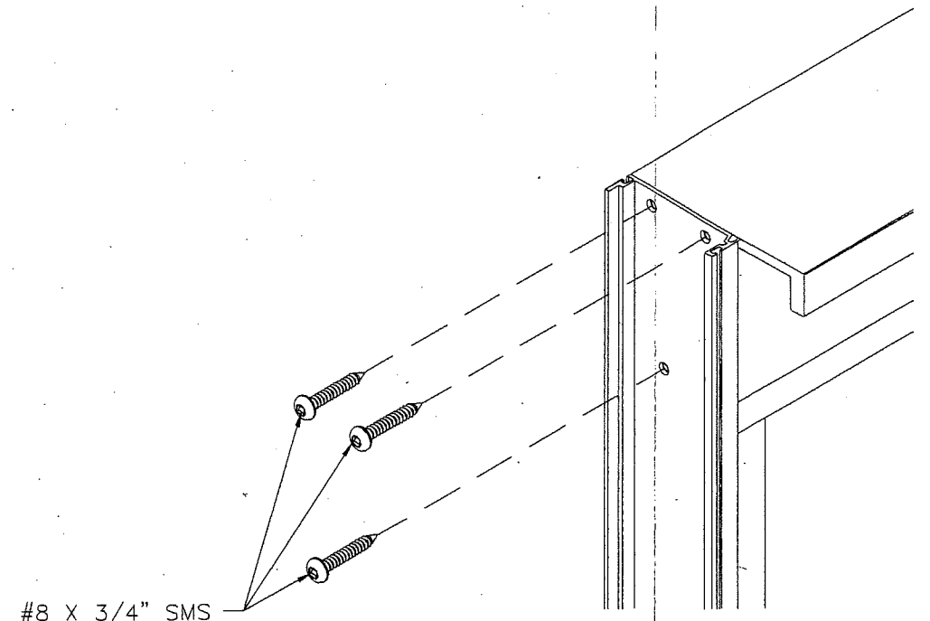
SASH CORNER DETAIL
