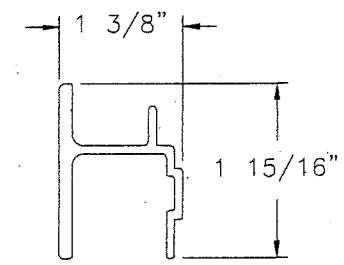
36 REINFORCEMENT ALUMINUM 6005-T61 .090" THICK
