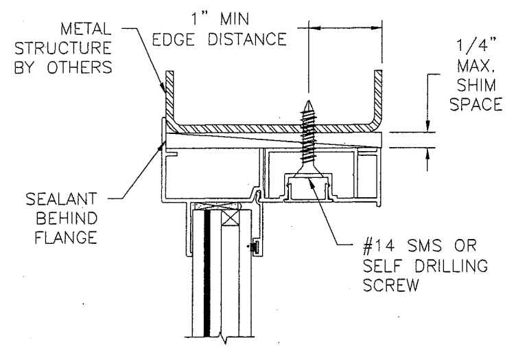
VERTICAL CROSS SECTION METAL STRUCTURE INSTALLATION
