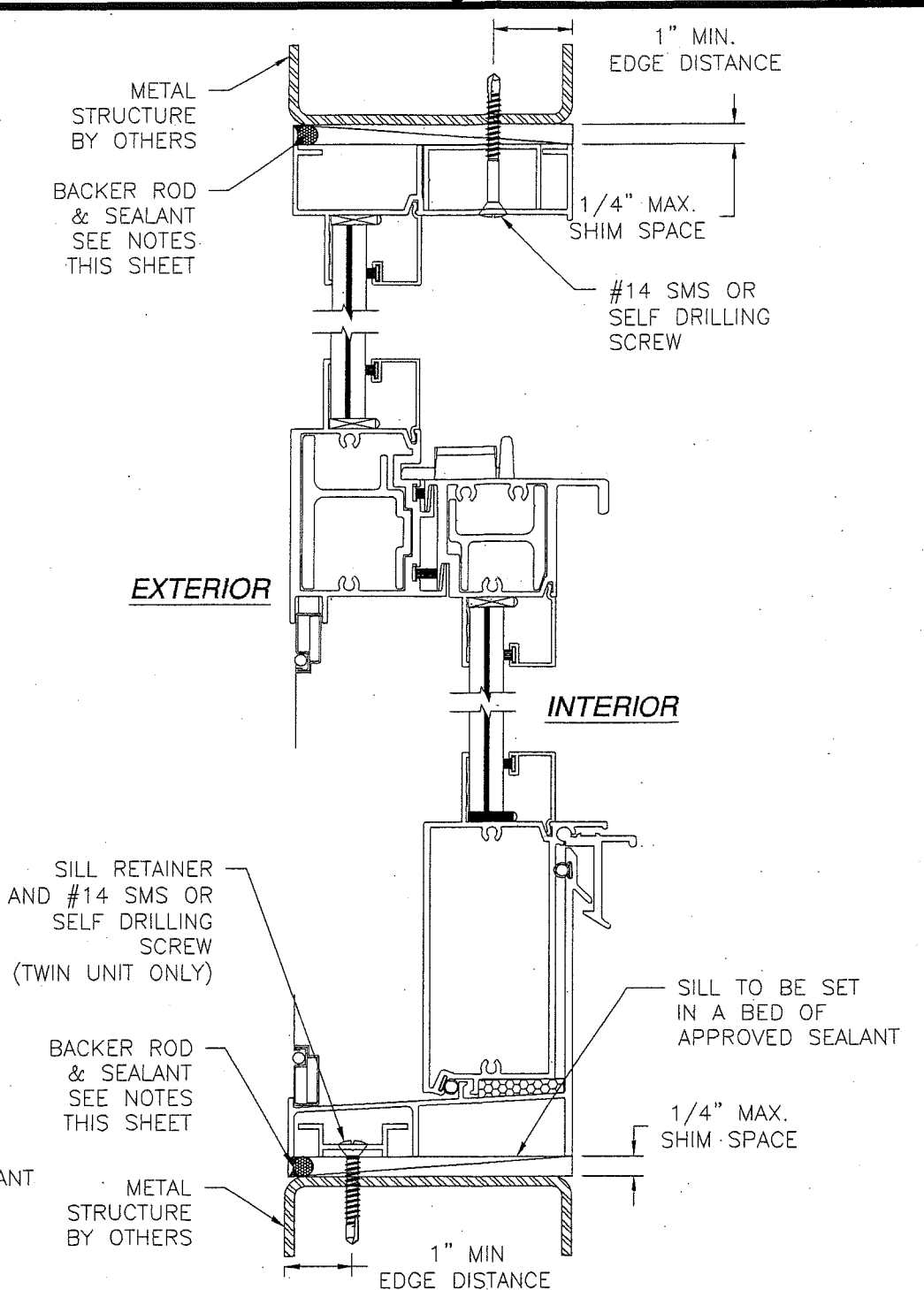
A/7 VERTICAL CROSS SECTION METAL STRUCTURE INSTALLATION
