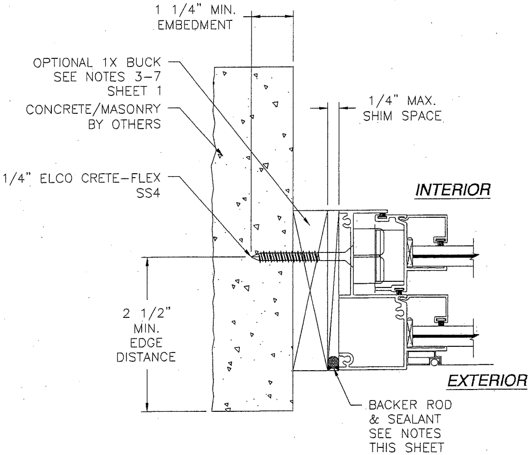
B 8 JAMB INSTALLATION DETAIL CONCRETE/MASONRY INSTALLATION
