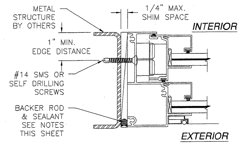
B/7 JAMB INSTALLATION DETAIL METAL STRUCTURE INSTALLATION
