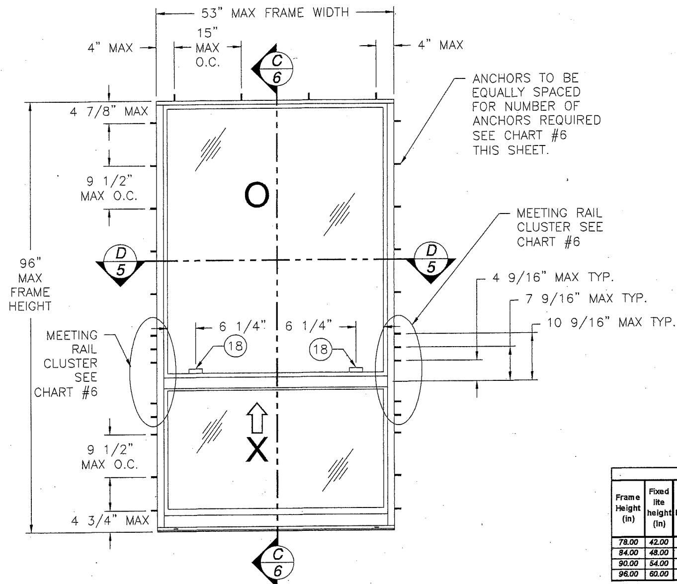
4000 ALUMINUM SINGLE HUNG ORIEL WINDOW EXTERIOR VIEW
