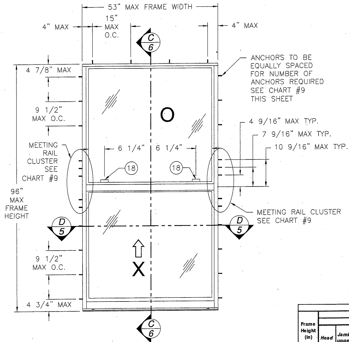
4000 ALUMINUM SINGLE HUNG WINDOW EXTERIOR VIEW
