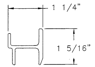
37 REINFORCEMENT ALUMINUM 6005-T61 .090" THICK
