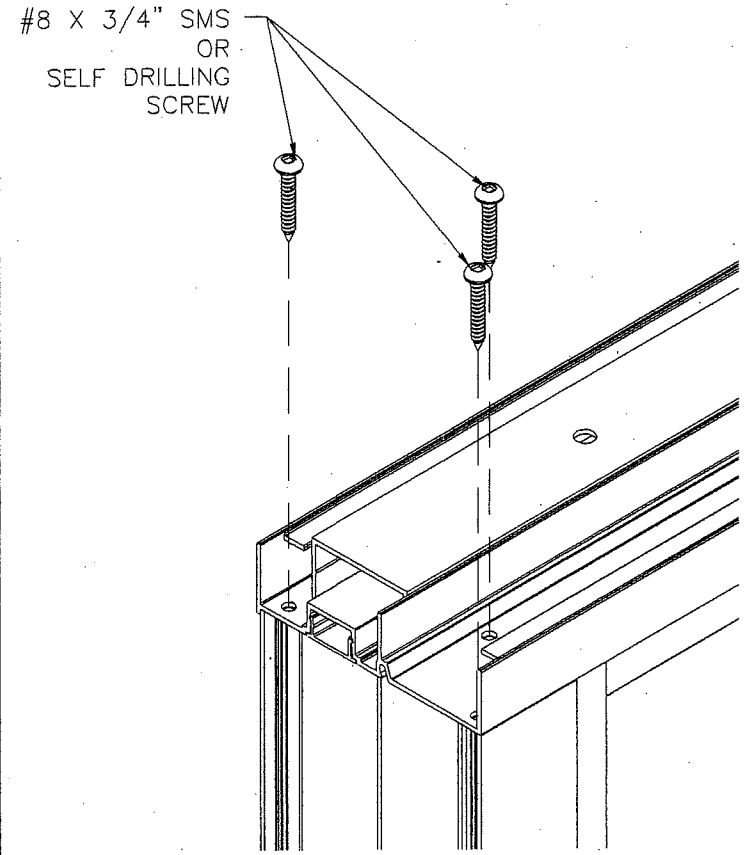
FRAME CORNER DETAIL
