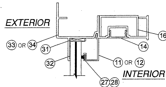
OPTIONAL HEAD FLANGE FRAME
