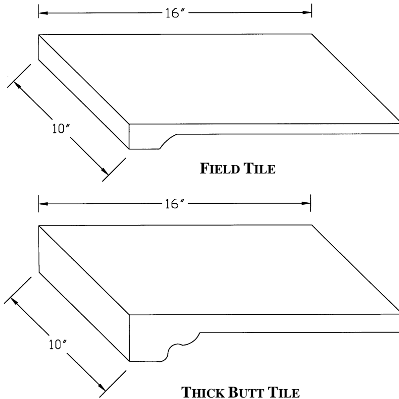
PROFILE DRAWING Bermuda "FLAT" CONCRETE ROOF TILE
