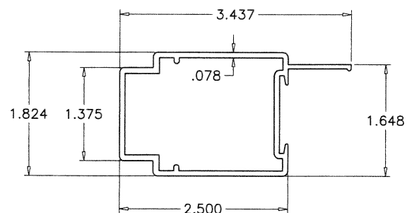
⑧ PANEL MALE ASTRAGAL
