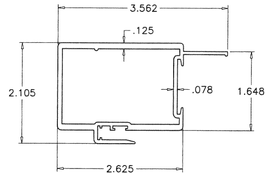
⑦ PANEL INNER INTERLOCK
