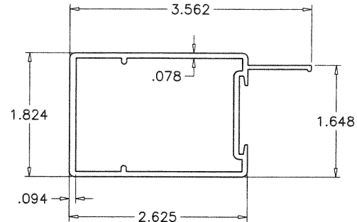
⑤ PANEL LOCK STILE
