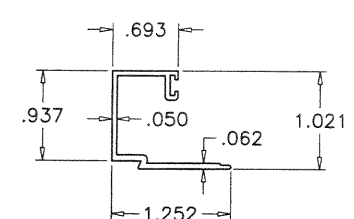
⑪ GLAZING BEAD 7/16" LAM. GLASS
