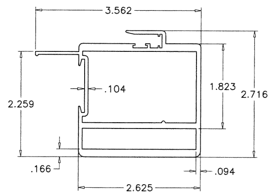
⑥ PANEL OUTER INTERLOCK
