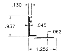
⑩ GLAZING BEAD 1" INSUL. LAM. GLASS
