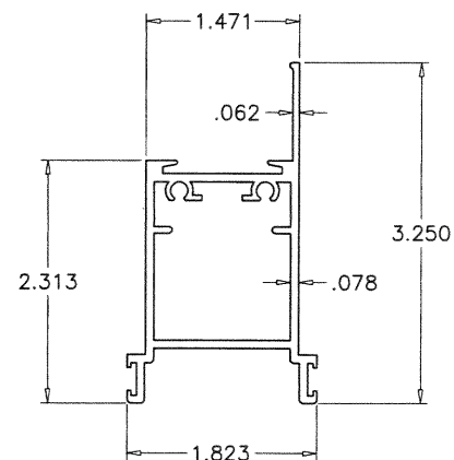
④ PANEL TOP & BOTTOM RAIL
