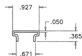
⑭ FRAME SILL COVER
