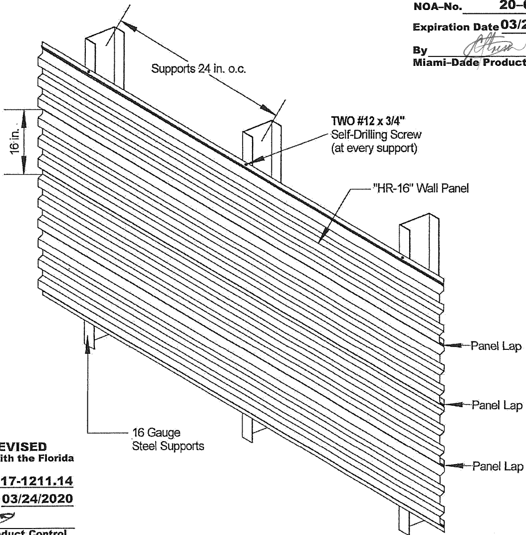
TYPICAL ELEVATION VIEW OUTSIDE OF WALL ASSEMBLY
