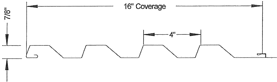
TYPICAL PANEL PROFILE
