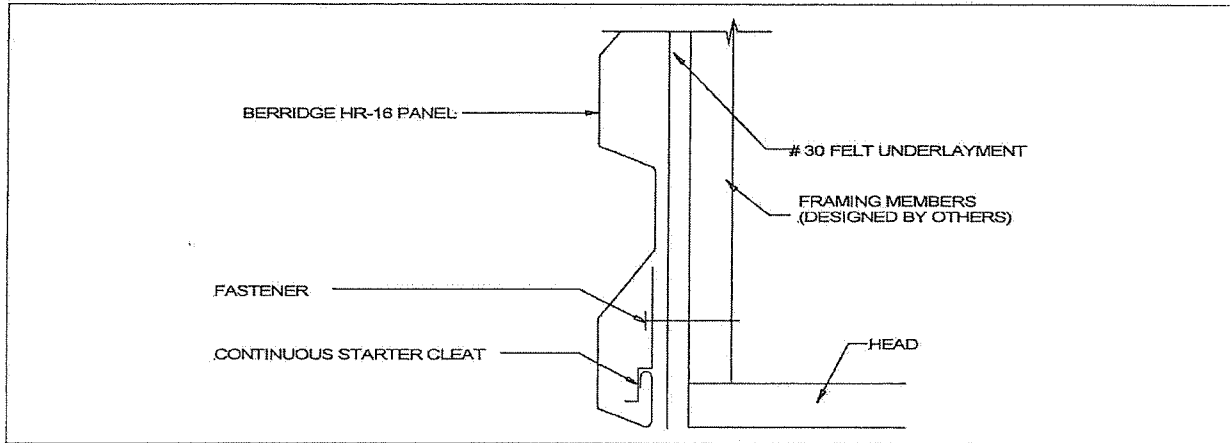
TYPICAL HEADER DETAIL
