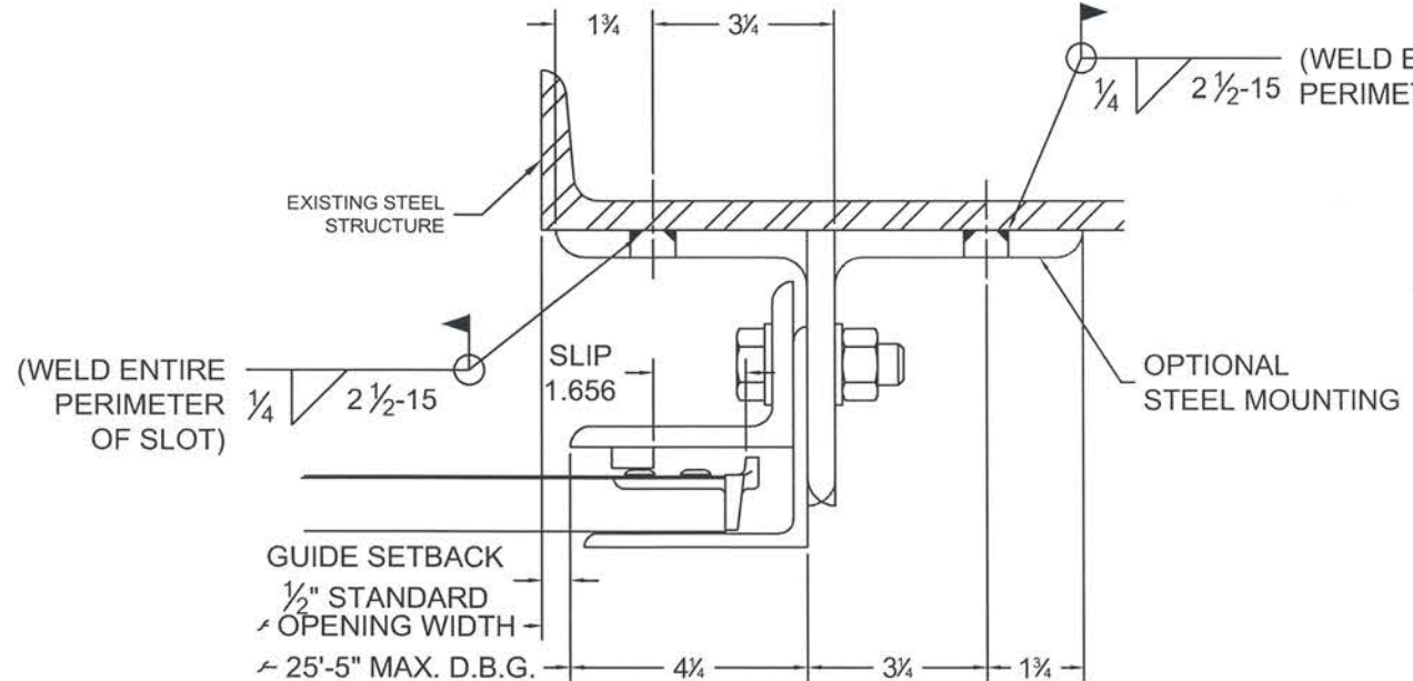
⑩ GUIDE ASSEMBLY STEEL STRUCTURE (Z-GUIDE OR E-GUIDE)
