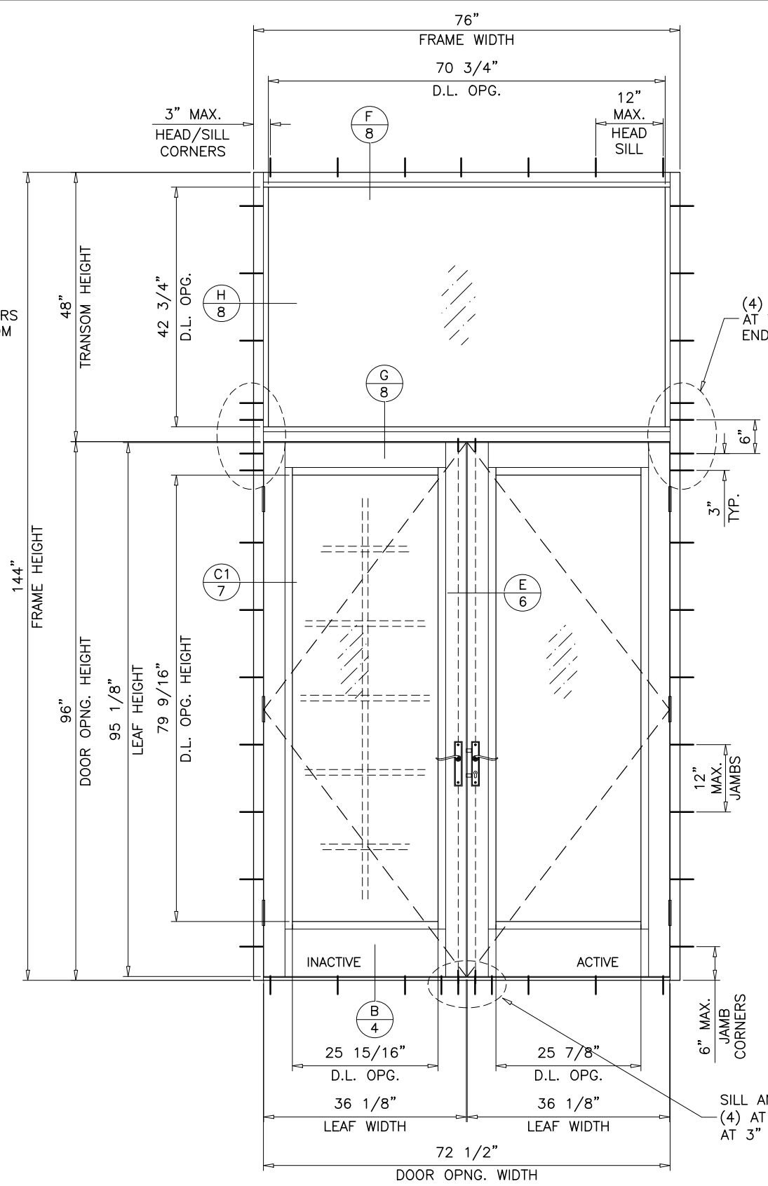
TYPICAL ELEVATIONS
