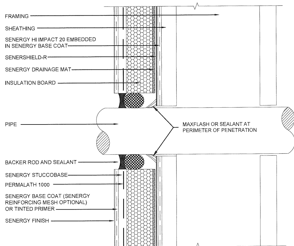
PIPE PENETRATION
