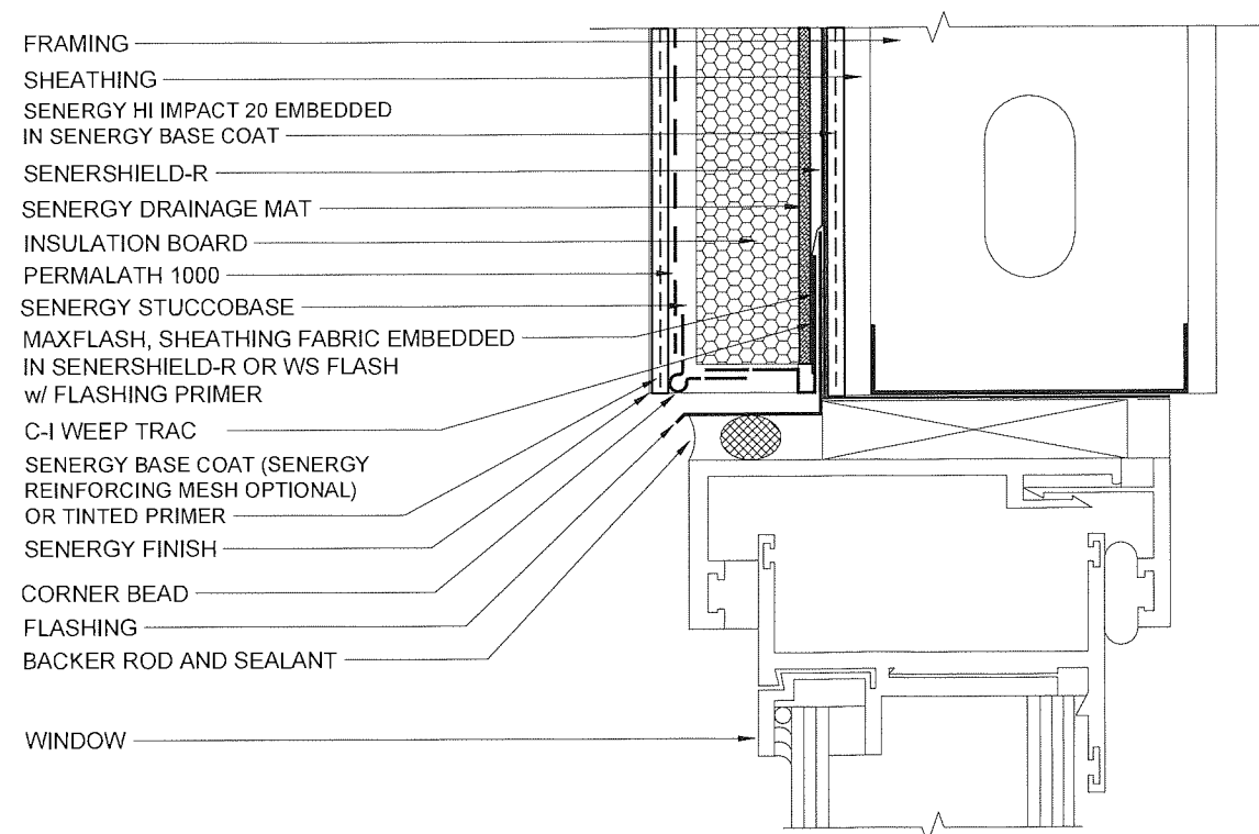
WINDOW HEAD (FLUSH)
