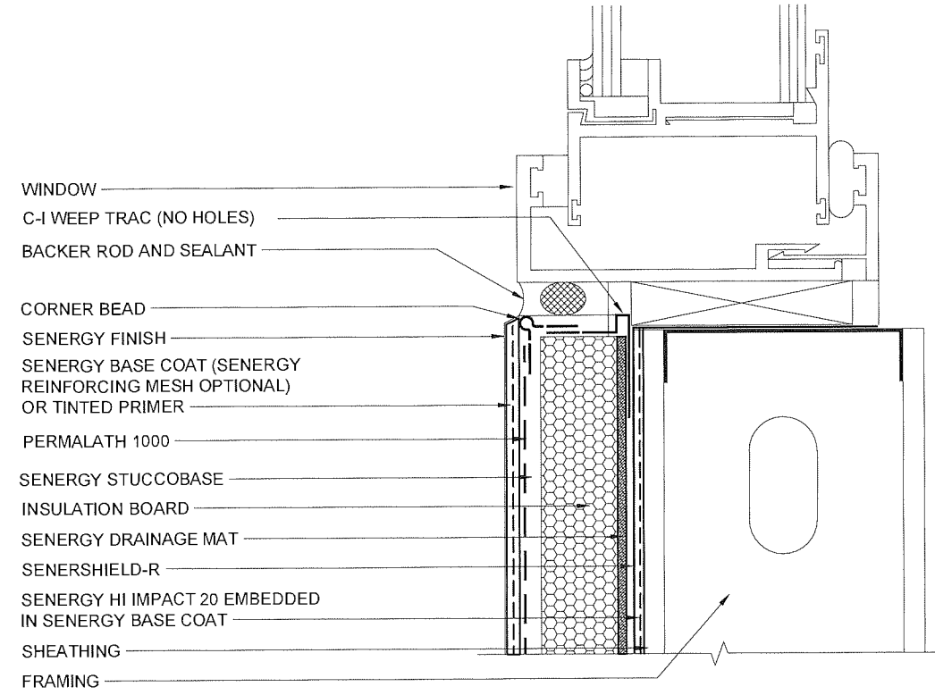
WINDOW SILL DETAIL (FLUSH)
