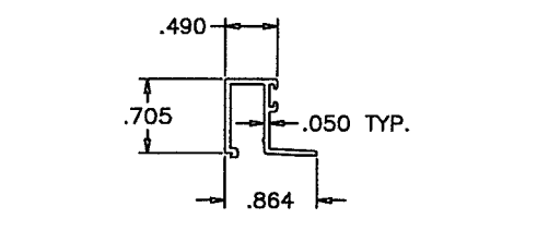
E8 5/16" GLAZING BEAD
