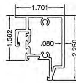
606-Moving Intlck. 6063-T6
