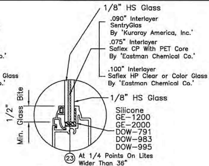
Glass Type "2" 5/16" Nominal Glass HS/HS
