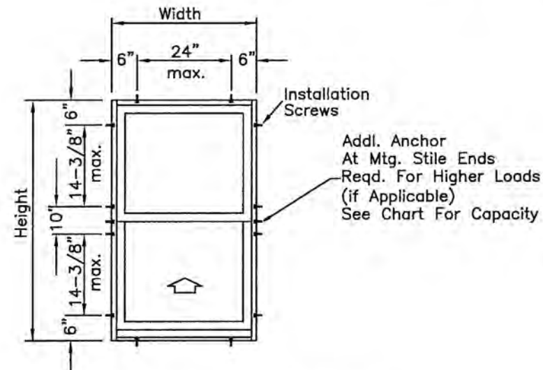
WinDoor Standard Hole Pattern
