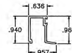
630-Glzg. Bead 6063-T6 For Glass Types 3 & 3A
