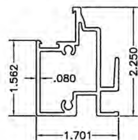
605-Fixed Intlck. 6063-T6
