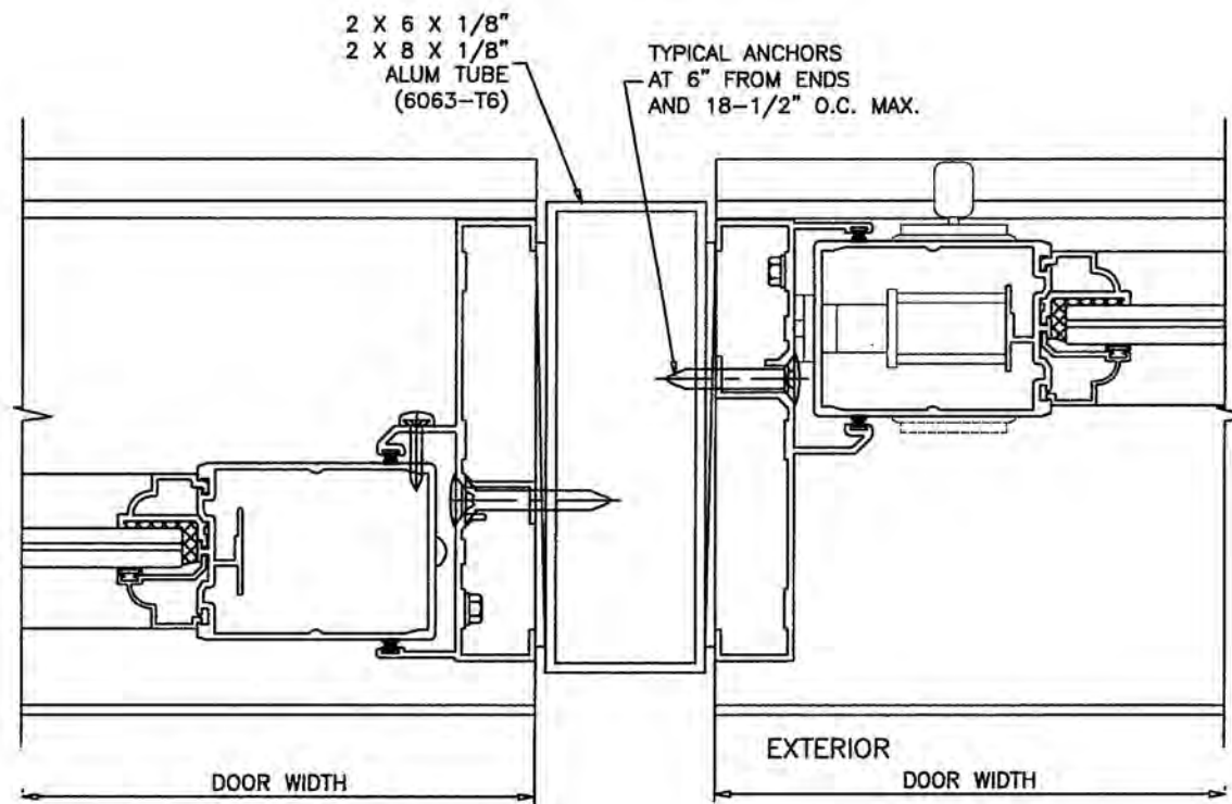
UNCLIPPED MULLION
