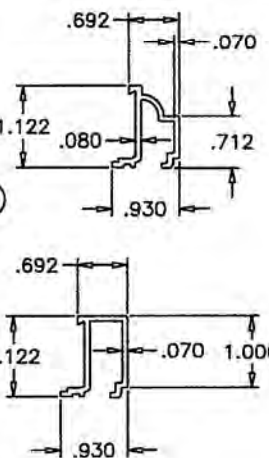
⑪A GLASS ADAPTERS
