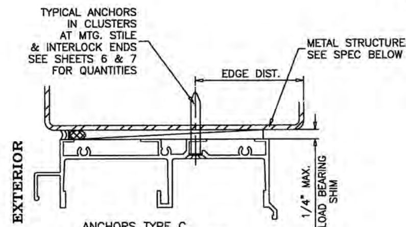
ANCHORS TYPE C INTO METAL STRUCTURES OR APPROVED MULLIONS
