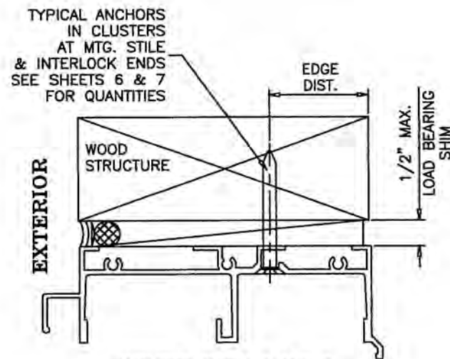
ANCHORS TYPES A AND D INTO WOOD STRUCTURES
