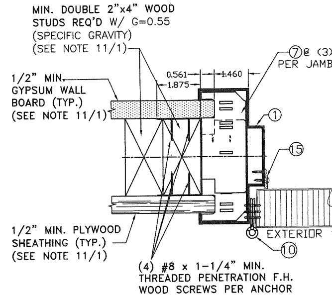
SECTION E
