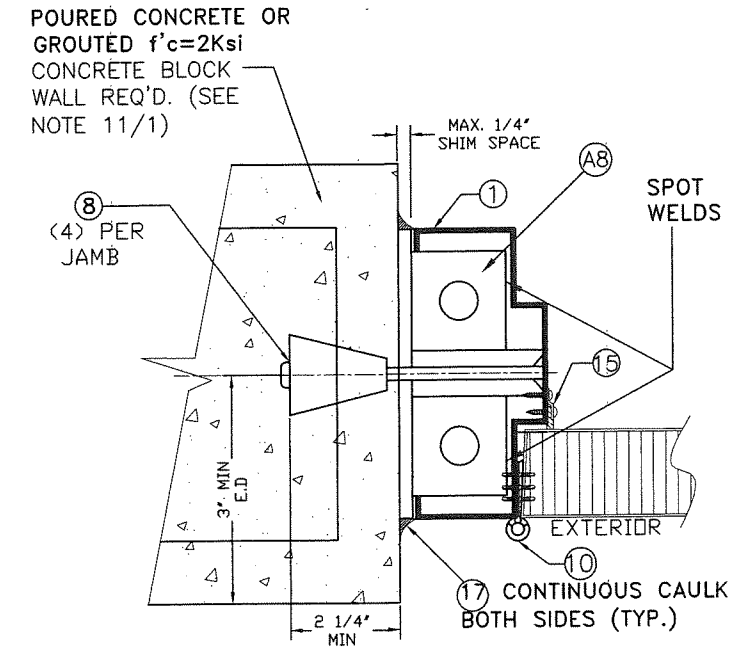
SECTION F
