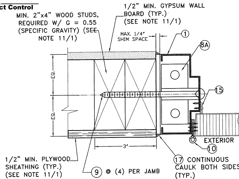
SECTION G
