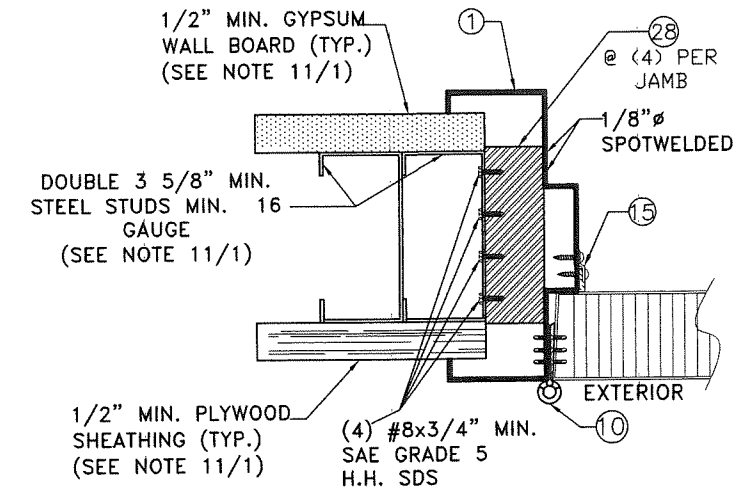
SECTION H
