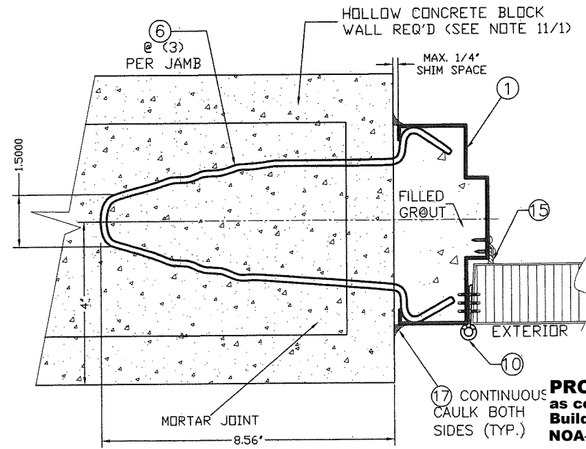
SECTION C
