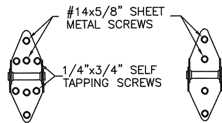
14 GA. END HINGES VIEW "B" 14 GA. INTERMEDIATE HINGE VIEW "C"
