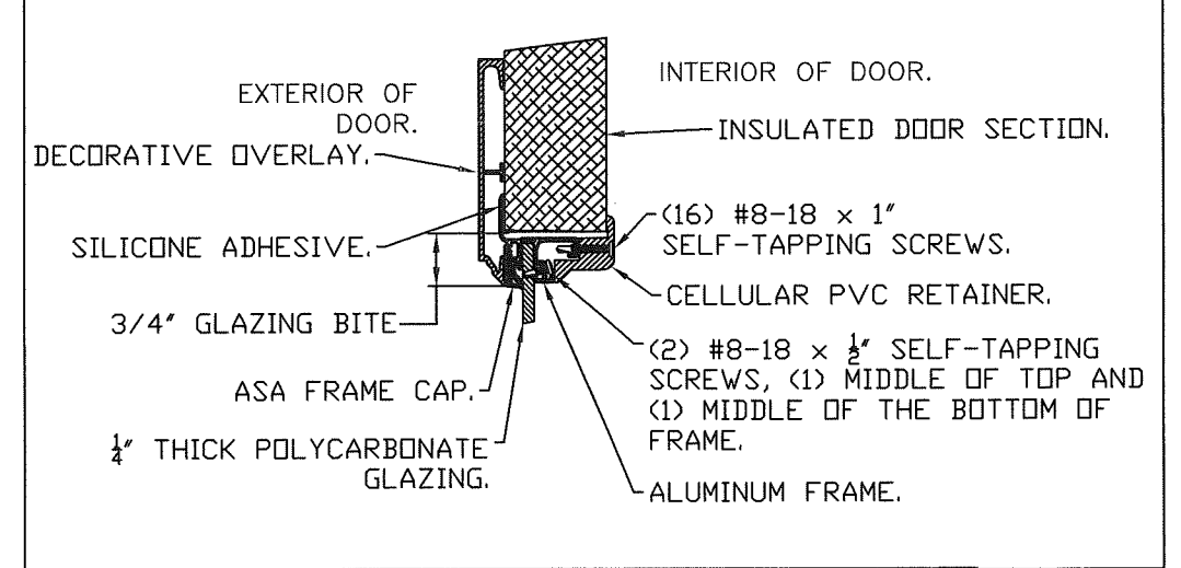
IMPACT-RESISTANT GLAZING DETAILS
