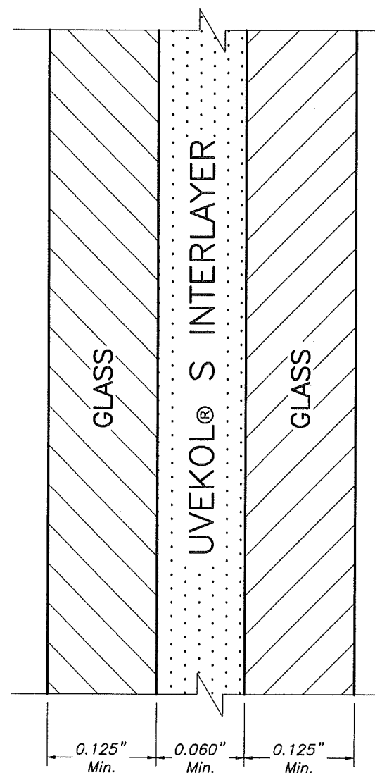
CROSS SECTION
