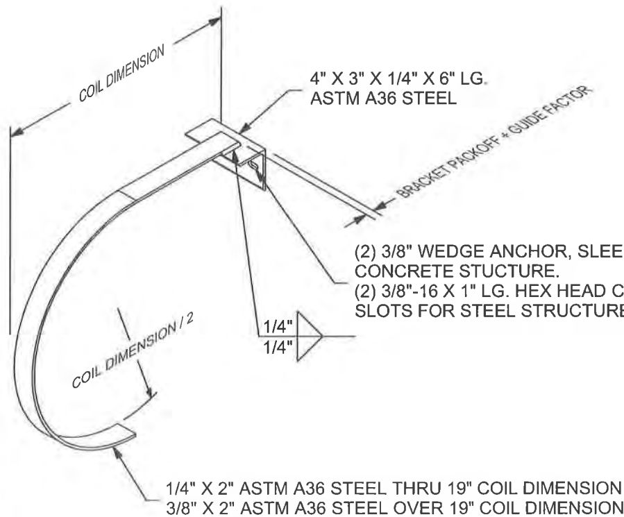
15 MID-HOOD SUPPORT (WHEN REQUIRED) "D" SHAPE DEPICTED, SQUARE STYLE ALSO AVAILABLE SCALE 3/32
