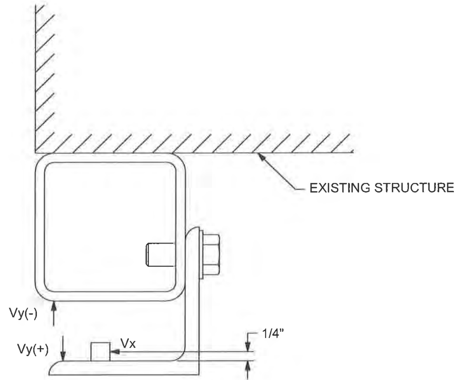
10 SUPERIMPOSED LOAD DIAGRAM - BOX GUIDE SCALE 3/8
