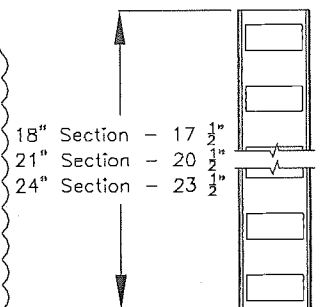
DETAIL K
