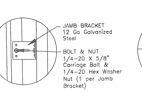
DETAIL F
