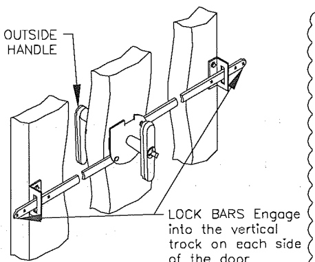
DETAIL J
