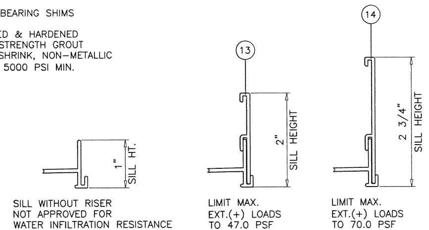
SILL HEIGHTS VS WATER RESISTANCE EXT.(+) LOAD
