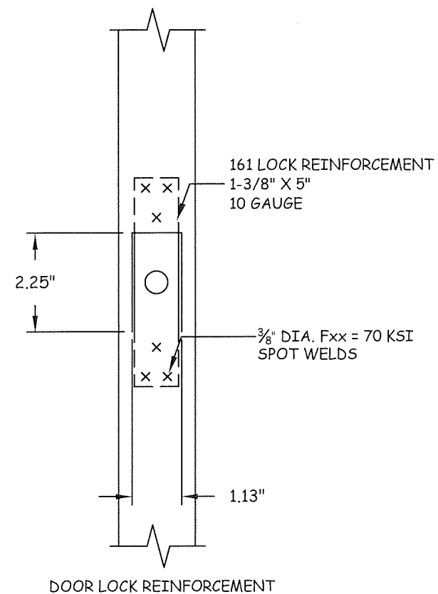
DOOR LOCK REINFORCEMENT
