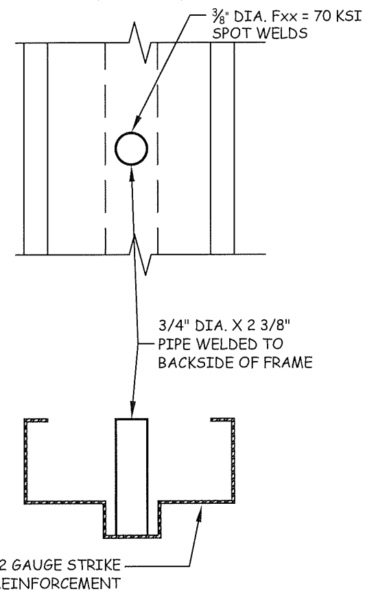
12 GA. STEEL REINFORCED DOOR FRAME
