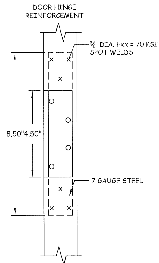
⑪ DOOR HINGE REINFORCEMENT
