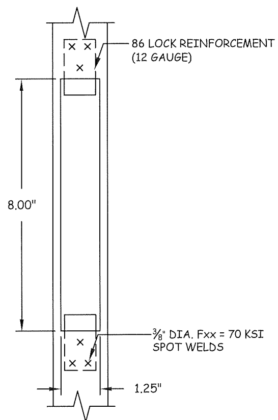
② DOOR LOCK REINFORCEMENT
