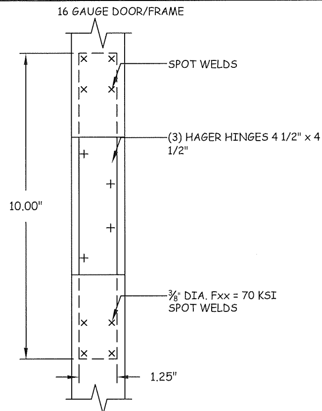
⑪ DOOR & FRAME STEEL HINGE PLATE 7 GAUGE x 1 1/4" x 10"
