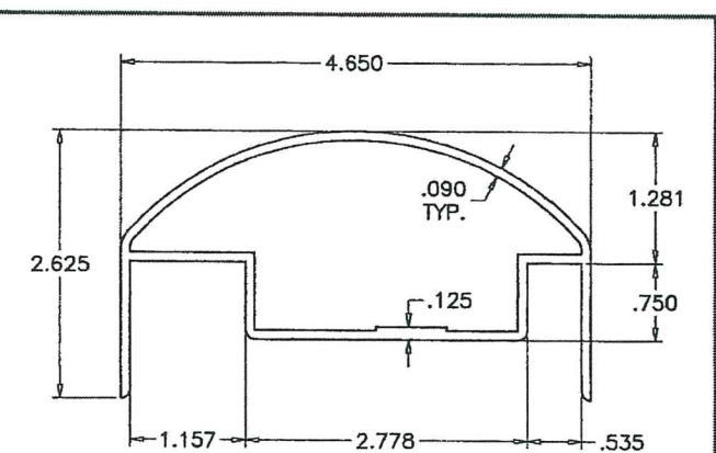
① TOP RAIL CAP
