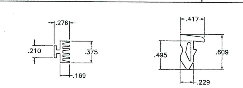
⑦ EXTERIOR GLAZING GASKET SCALE 1:1 ⑧ INTERIOR GLAZING GASKET SCALE 1:1
