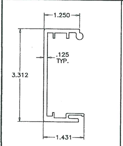
④ FEMALE POST
