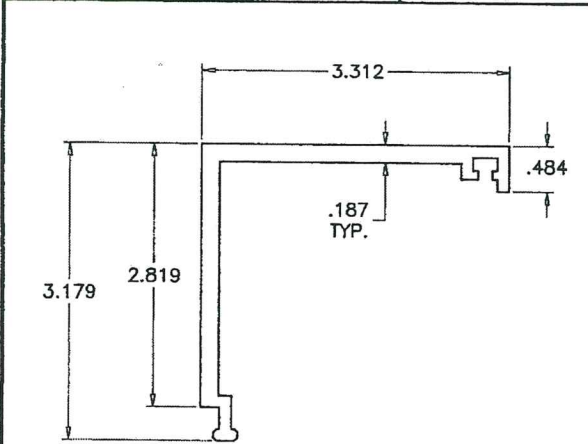
⑥ CORNER POST
