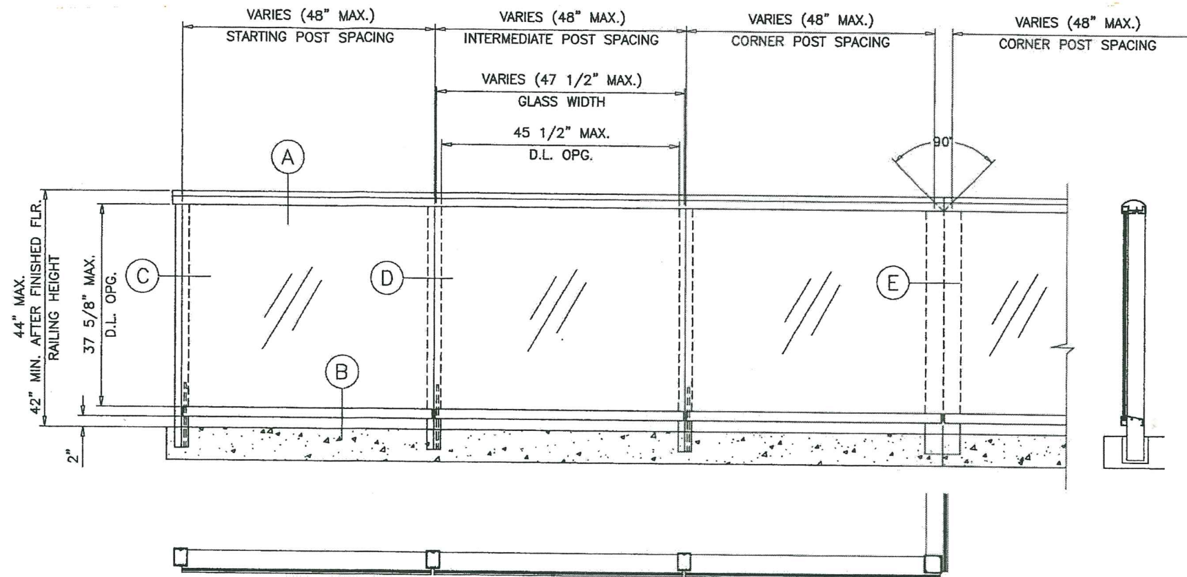
TYPICAL ELEVATION
