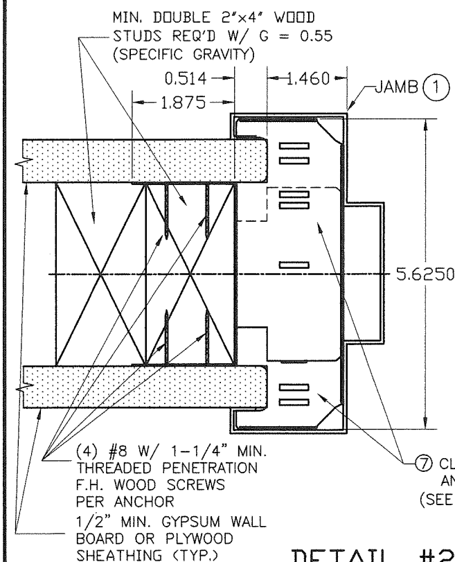
DETAIL #21 WIRE ANCHOR ⑥ INSTALLATION TO MASONRY WALLS
