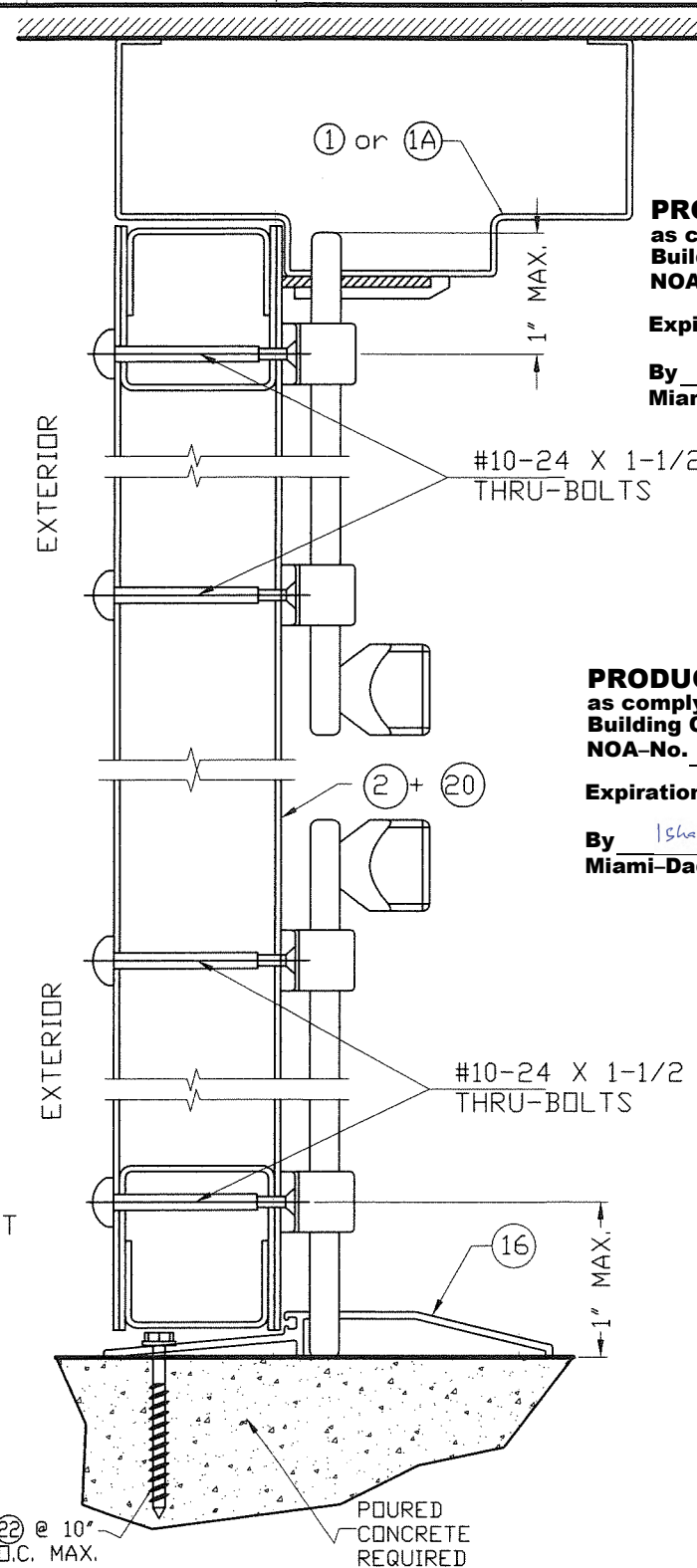
TYPICAL SECTION
