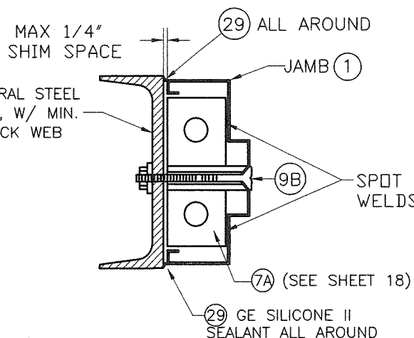
DETAIL #23A INSTALLATION OF 3/8"Ø F.H. M.S. ⑨B TO STEEL CHANNEL
