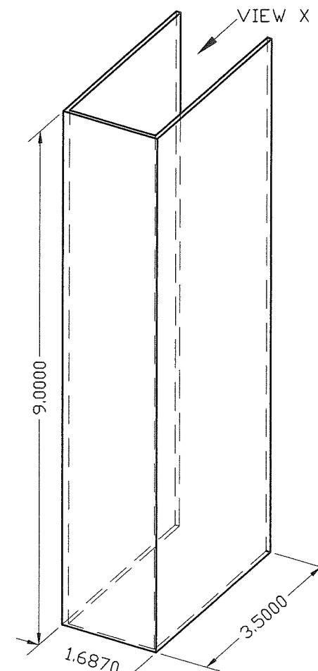
3D VIEW
