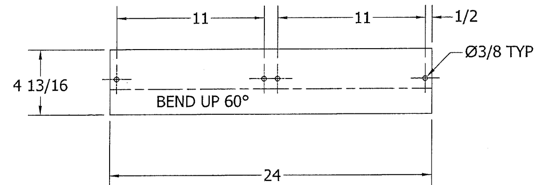
SECTION RAIL SPLICE
