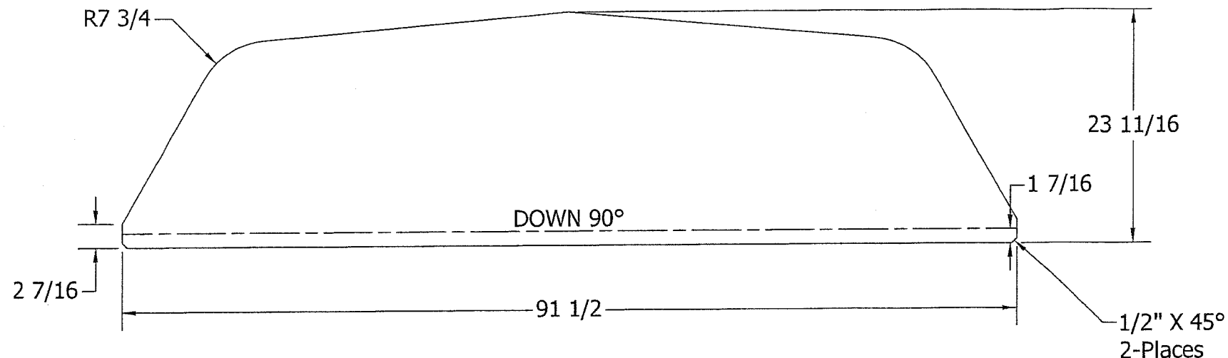
HOOD END PANEL
