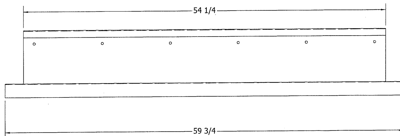
BASE PANEL *PUNCH HOLES IN TWO PARTS ONLY
