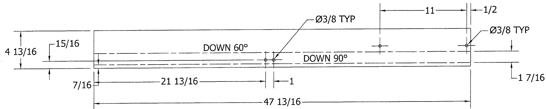
SECTION RAIL
