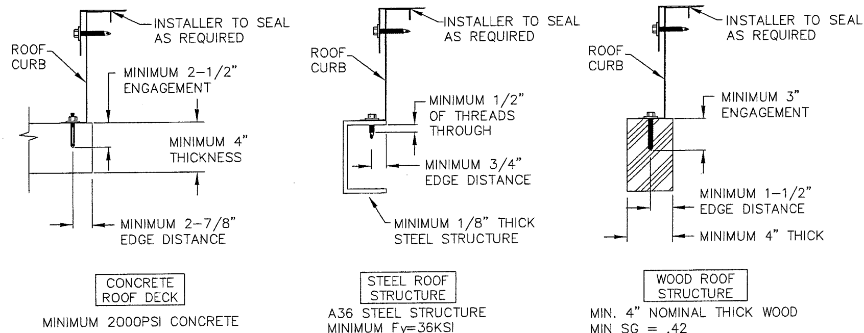
ATTACHMENT OF CURB TO ROOF STRUCTURE
