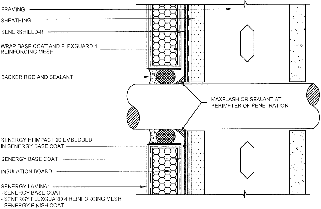
PIPE PENETRATION
