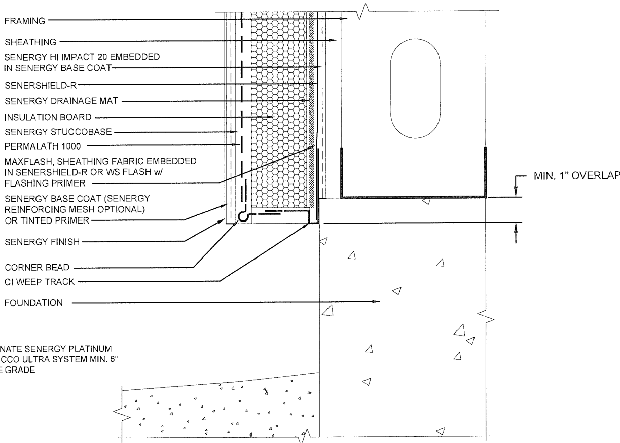
TERMINATION AT FOUNDATION
