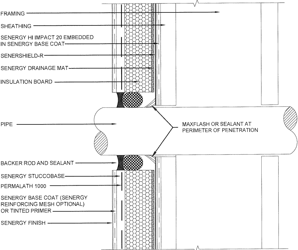
PIPE PENETRATION
